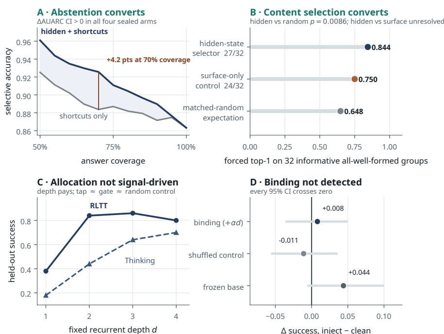
Figure 13. Four of the five sealed conversions, drawn. (A) C1: hidden-plus-shortcut scores dominate the shortcut-only risk-coverage curve on pooled Horizon (4-shortcut arm; +4.2 points of selective accuracy at 70% coverage), and the \Delta\text{AUARC} interval excludes zero in all four sealed arms. (B) C4: on the all-well-formed pool the hidden-state selector clears the exact matched-random null (27/32, p = 0.0086 ); the surface-only control also beats random, and the hidden-vs-surface increment is unresolved. (C) C2: the fixed-depth tables show large returns to recurrent depth on both checkpoints (with RLTT’s d_3 \geq d_4 non-monotonicity) — yet neither the tap allocator nor the native exit gate beats a matched-histogram random control at any budget, so which tasks get the depth carries no detectable signal. (D) C5: the sign-conditioned LoRA’s injection effect is indistinguishable from its shuffled control, and the frozen re-measure reproduces §8.1’s no-reliable-effect. C3, the prefix-prune tournament, is not drawn: its pool could not be powered (0.978 any-of-6 ceiling). Full tables for all five in Appendix L.
