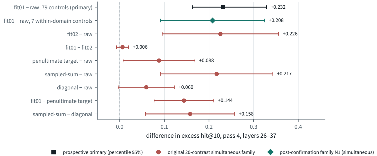
Figure 4: Pass-4 band contrasts; the dashed vertical line marks zero difference. Black square: the prospective primary (percentile interval). Red circles: contrasts of the original 20-member simultaneous family. Teal diamond: the post-confirmation within-domain-control contrast (Section 4.4, family N1).
