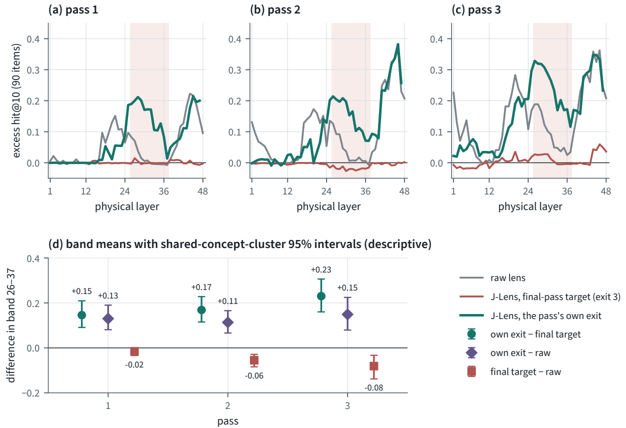
Figure 5: Application-era matched banks (same recipe, target differs) evaluated on the discovery population, fixed layers, passes 1–3: raw lens (grey), final-target J-Lens (red) and the pass’s own-exit J-Lens (teal). (d) Band means with descriptive shared-concept-cluster 95% intervals. Post hoc and descriptive; not the confirmation population.
