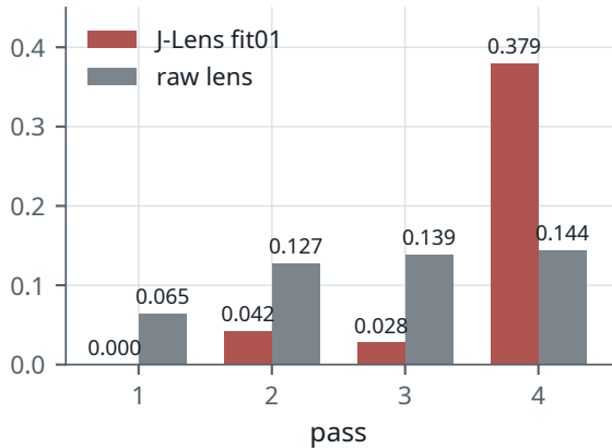
(b) intended-concept recovery
