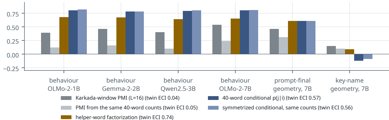
Spearman \rho over 105 key pairs
