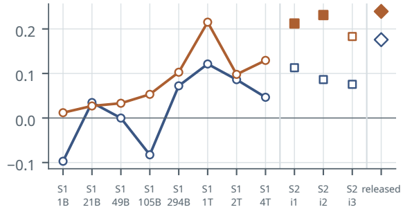
(b) residual correspondence with corpus conditionals
