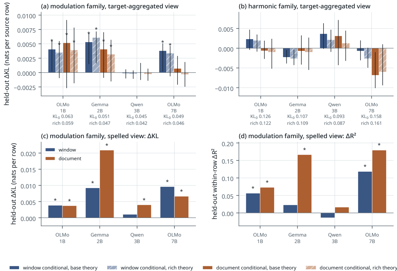
Figure 6. Held-out gain from the corpus conditionals beyond the theory model, Wikipedia. (a, b) Target-aggregated view: reduction in held-out KL per source row when the corpus row is added to the theory features, for the window (blue) and document (orange) conditionals, with the base (solid) and rich (hatched) theory model; each tick label gives the base and rich theory-only held-out KL, and hatched bars should be read against the rich value; *: relabeling p < .05 ; (a) modulation family, (b) harmonic-relation family. (c) Spelled view, modulation family, held-out \Delta\text{KL} ; (d) the same cells scored by within-row \Delta R^2 — under the corrected base model the two scorers disagree on significance in one of the eight target-aggregated modulation cells (OLMo-7B \times document) and in two of the eight spelled cells. Numbers in Appendix C.
