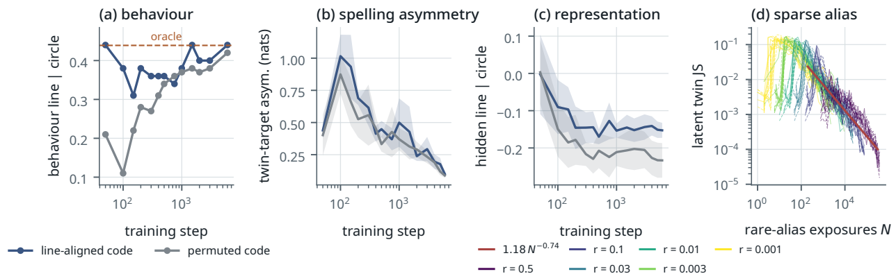
Figure E.1. Synthetic controls. (a–c) Periodic (CIRCLE) law, line-aligned vs permuted output code, five paired seeds: behaviour (line | circle without code control, seed means) reaches the oracle’s own value faster under the aligned code and ends at the same value (a); the spelling asymmetry between twin targets is transiently larger and vanishes (b, mean \pm sd); the predictive-state representation keeps a small persistent relative shift toward the line under the aligned code, both partials remaining negative and below their relabelling nulls (c, last layer, mean \pm sd; the headline +0.097 contrast is at the mid layer). (d) Sparse source aliases: latent twin divergence collapses onto one power law in cumulative rare-alias exposures across rarity levels r (solid: aligned code; dashed: permuted).
