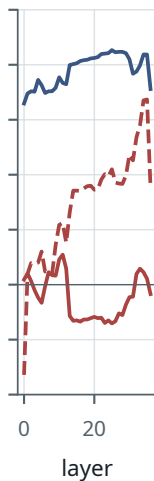
Qwen2.5-3B
