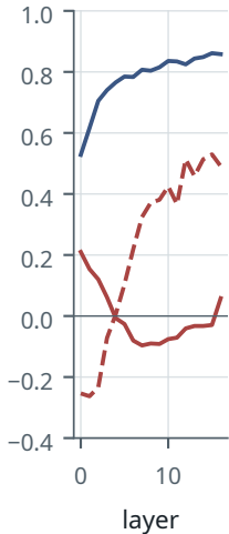
(b) OLMo-2-1B
