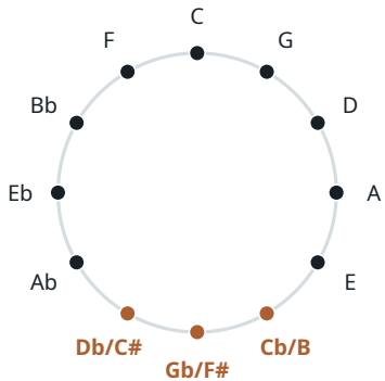
(a) neutral pitch classes: circle of fifths
