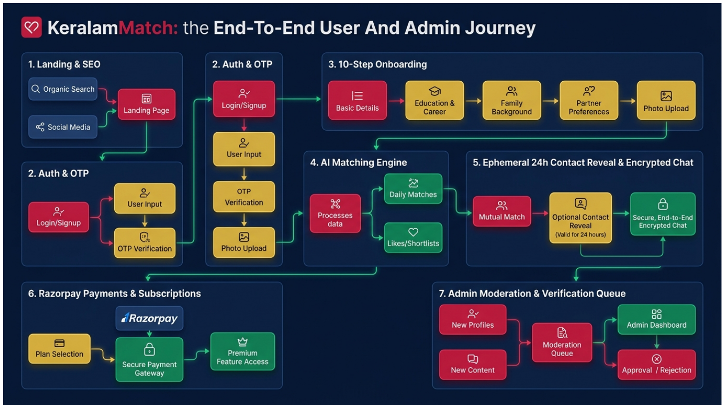
Figure 1: KeralamMatch End-to-End System Journey Flowchart
