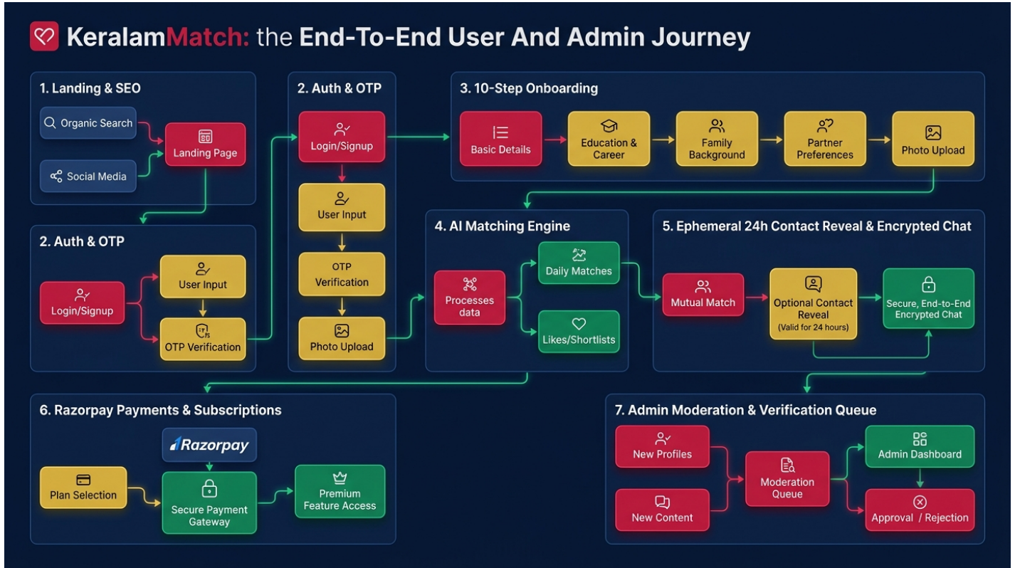
Figure 1: Keralamatch End-to-End User & Admin Journey Flowchart Diagram
