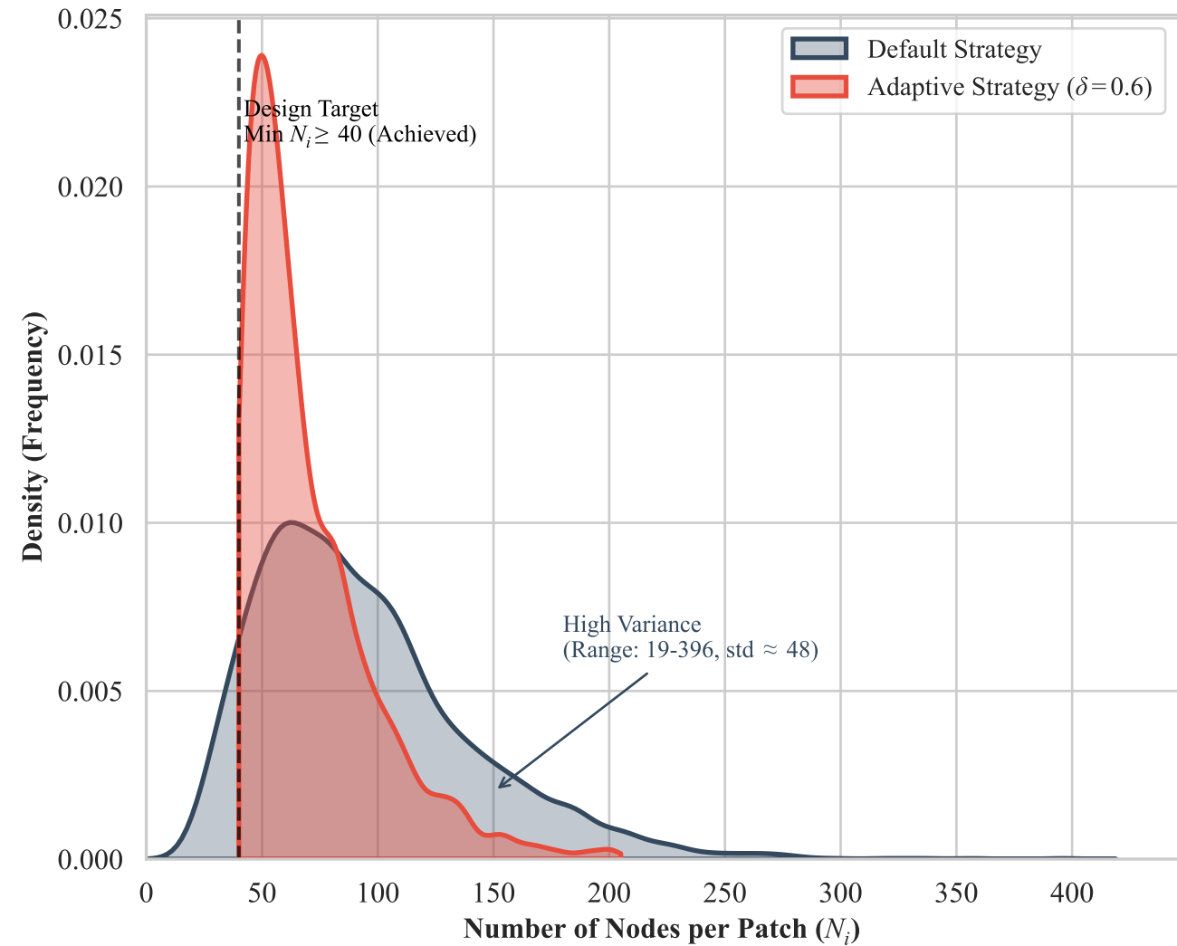
(B) Resulting Node Count Distribution per Patch (Simulated)
