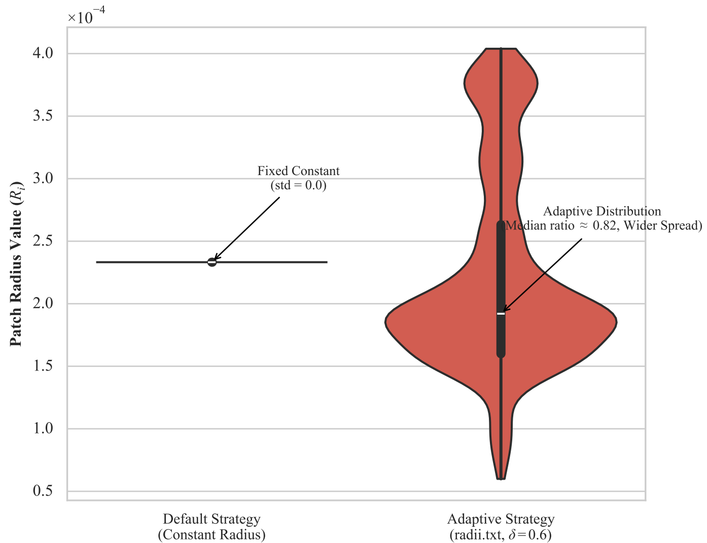
(A) Comparison of Patch Radius Strategies (Actual Data)
