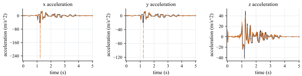
Figure 17: Ball-and-socket pendulum validation over 5 s: ball acceleration in the x , y , and z directions. Accelerations are shown as diagnostic channels for the contact transient; the displacement and velocity curves provide the primary trajectory-level validation because the three solvers use different contact regularizations and contact-envelope definitions.
