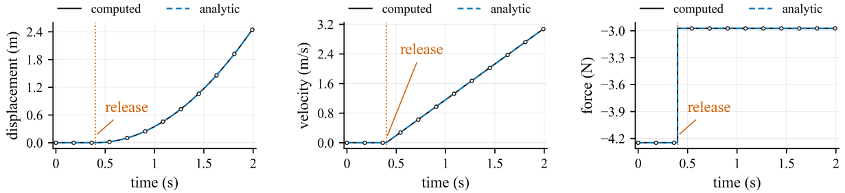
Figure 2: Release control on a 30^\circ inclined plane. The block is held until t = 0.40 s and then released; because the static capacity is exceeded, it switches to kinetic sliding and follows Eq. (43). The black computed curve and blue dashed analytic curve are plotted separately, with markers on the computed samples to keep the coincident curves distinguishable.
