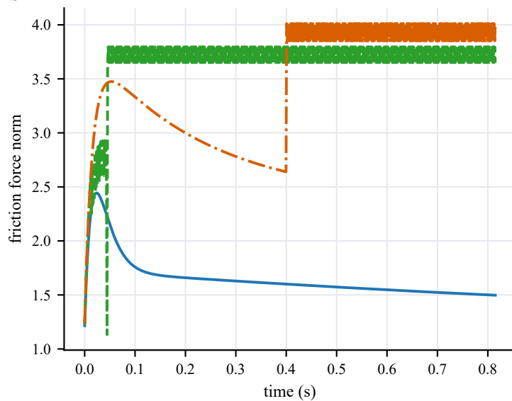
Same dynamic friction scene: wavy guide-slot ball head
