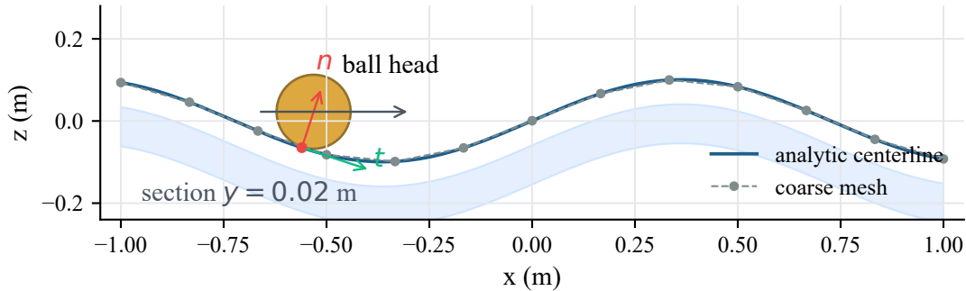
wavy guide-slot section
