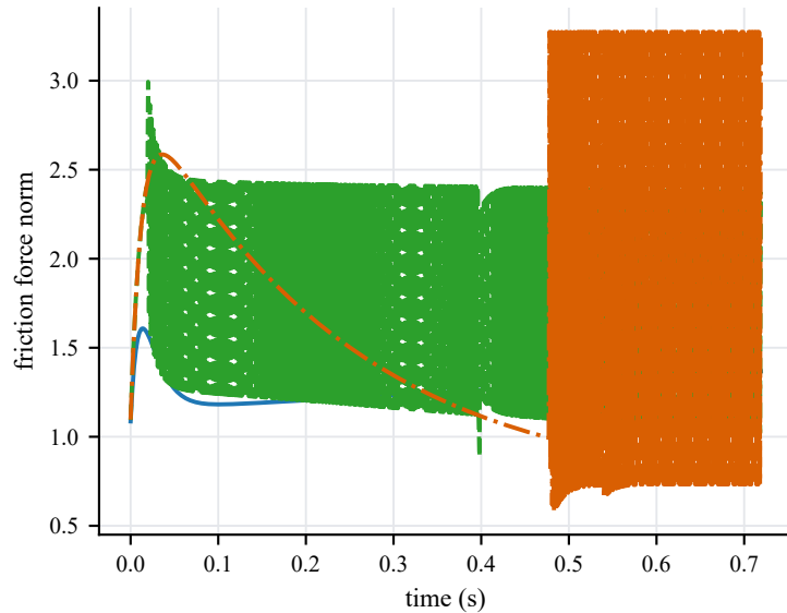
Cam-roller follower contact-geometry comparison
