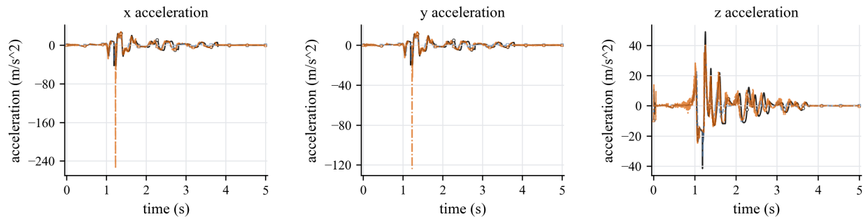
Figure 18: Ball-and-socket pendulum validation over 5 s: ball acceleration in the x , y , and z directions. Accelerations are shown as diagnostic channels for the contact transient; the displacement and velocity curves provide the primary trajectory-level validation because the three solvers use different contact regularizations and contact-envelope definitions.
