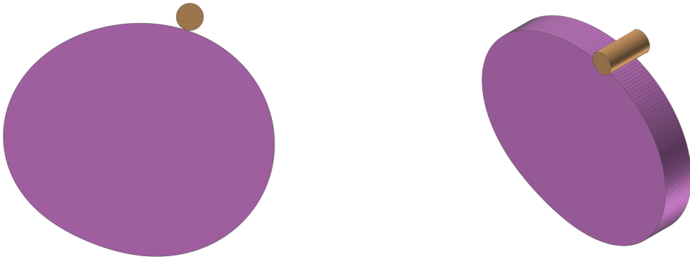
Figure 6: Cam-roller follower model configuration used for the contact-geometry comparison. The two views show the non-circular cam profile and roller follower geometry that produces sliding and rolling contact over a faceted collision representation.
