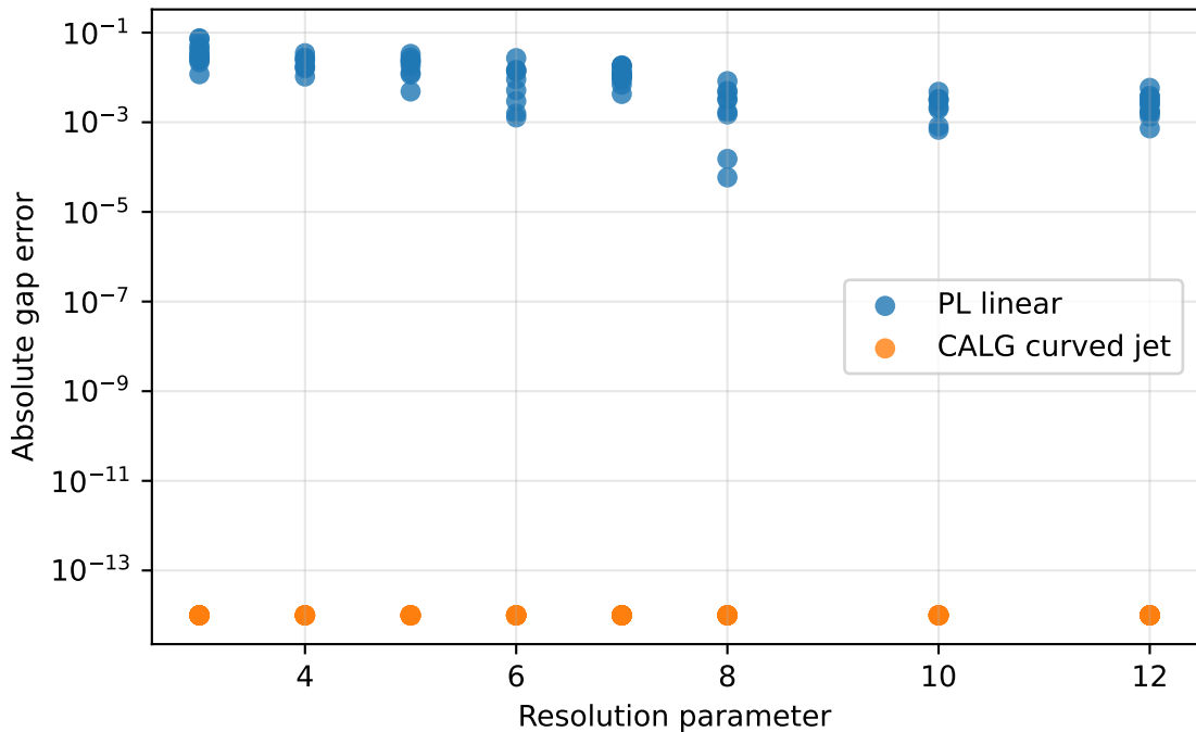
Randomized sub-cell smooth-contact statistics
