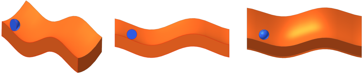
Figure 7: Model configuration for the Guide slot scene. The three views show the slot path, moving contact body, and contact geometry used by Recurdyn, Chrono, and CALG.
