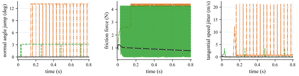
Figure 11: Independent contact-geometry comparison curves for the Ball-and-socket pendulum scene. The smooth CALG contact frame suppresses the high-frequency tangential-speed jitter and discrete friction-state changes observed in the fixed-tessellation baselines.
