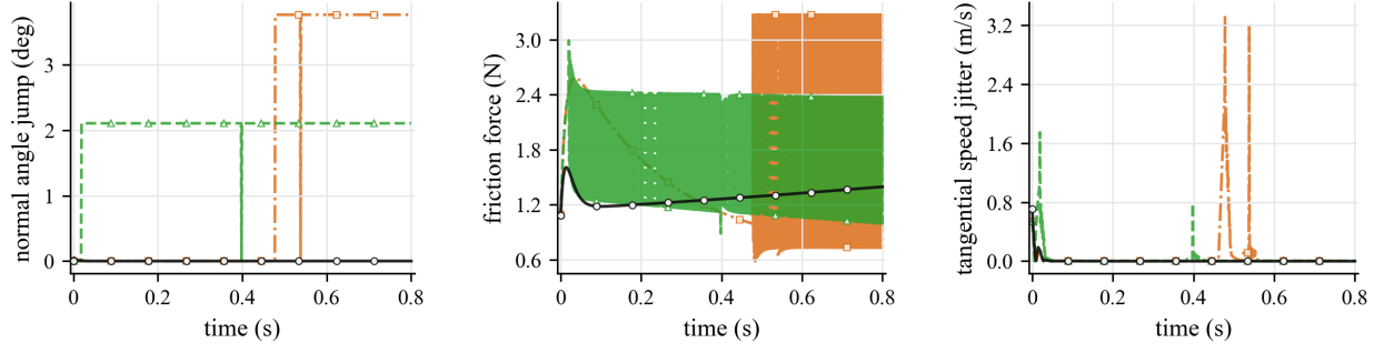
Figure 10: Independent contact-geometry comparison curves for the Cam-roller follower scene. Linear-triangle BVH and PN-triangle BVH produce larger normal and friction-force variations when the contact point traverses cam cells.
