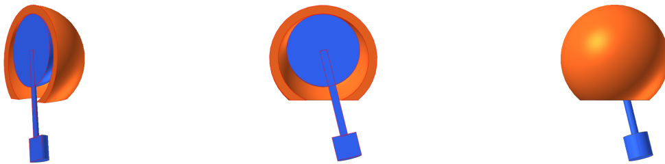
Figure 8: Model configuration for the Ball-and-socket pendulum scene. The three views show the socket, moving contact ball, and attached pendulum body used by Recurdyn, Chrono, and CALG.
