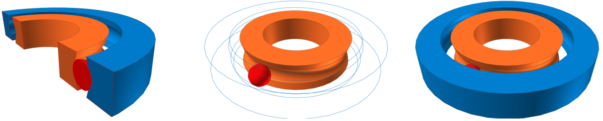
Figure 5: Model configuration for the Bearing raceway scene. The three views show the imported raceway geometry and rolling element configuration used by Recurdyn, Chrono, and CALG.
