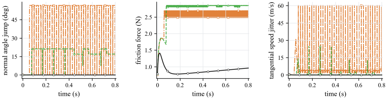
Figure 9: Independent contact-geometry comparison curves for the Bearing raceway scene. The body state, timestep, penalty stiffness, friction coefficient, and regularized Coulomb update are identical; only the contact-geometry module changes.
