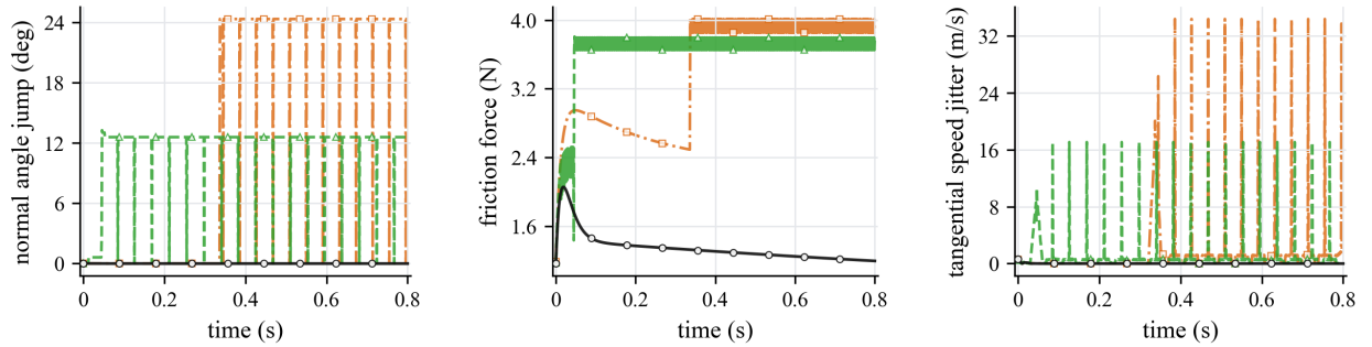
Figure 12: Independent contact-geometry comparison curves for the Guide slot scene. Cell-crossing normal changes in the Linear-triangle BVH and PN-triangle BVH modules enter directly into friction-force and tangential-speed jitter.
