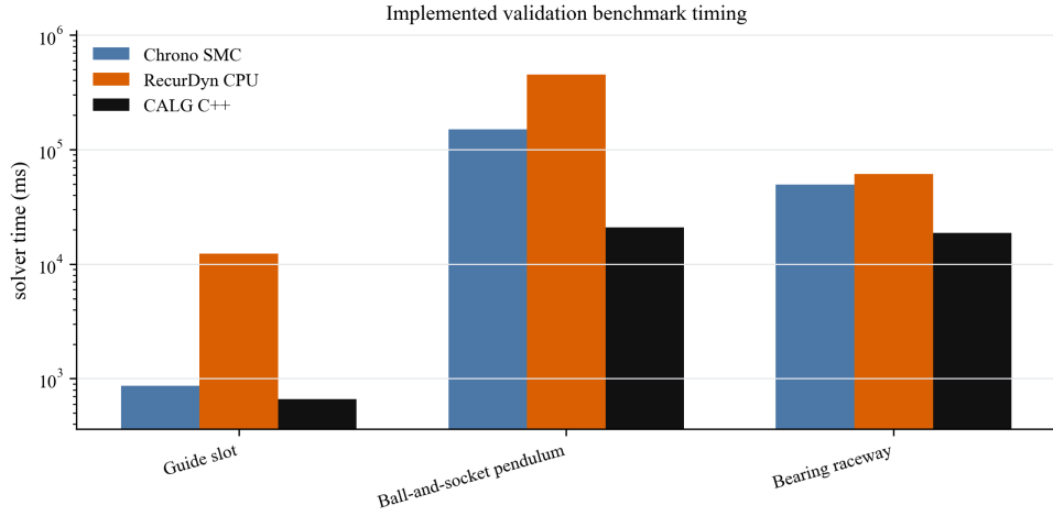
Figure 23: Solver timing per selected validation scene. CALG uses no-CSV solver-loop time and excludes one-time geometry preprocessing such as dense SDF construction; Recurdyn uses solver-reported CPU Time. All three CALG rows include local mesh/CALG detector traversal, configuration-space SDF signed refinement, and normalized surface-contact response quadrature. Timing ratios are reported in Table 6 and describe this implemented validation benchmark only, not a solver-wide engine comparison.
