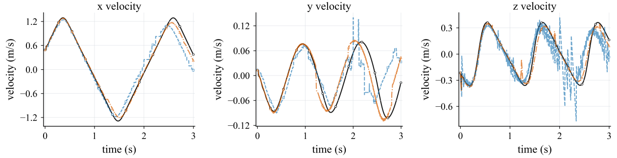
Figure 15: Guide slot validation over 3 s: ball velocity in the x , y , and z directions. The CALG result is shown as the black solid curve.
