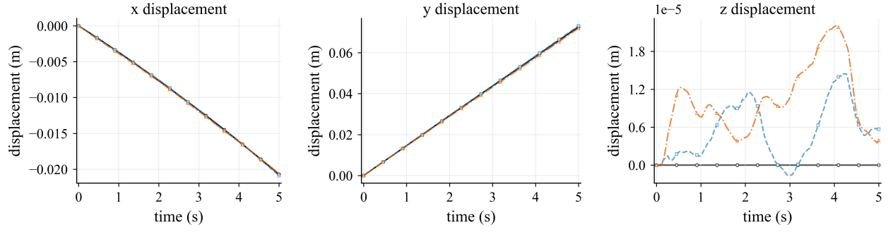
Figure 20: Bearing raceway validation over 5 s: ball displacement in the x , y , and z directions. The CALG result is shown as the black solid curve; displacements are relative to each solver's initial ball coordinate.
