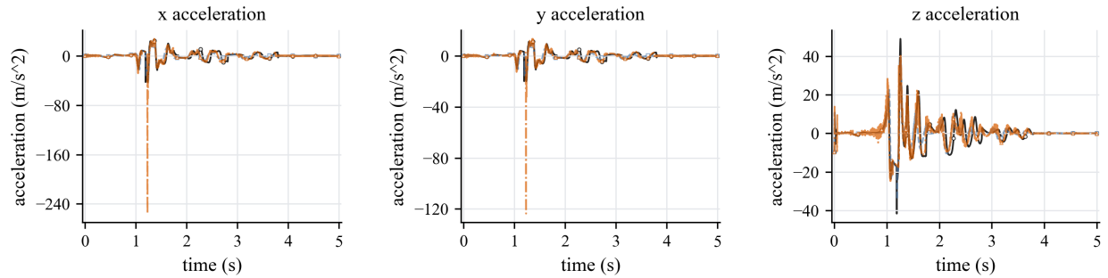
Figure 19: Ball-and-socket pendulum validation over 5 s: ball acceleration in the x , y , and z directions. Accelerations are shown as diagnostic channels for the contact transient; the displacement and velocity curves provide the primary trajectory-level validation because the three solvers use different contact regularizations and contact-envelope definitions.
