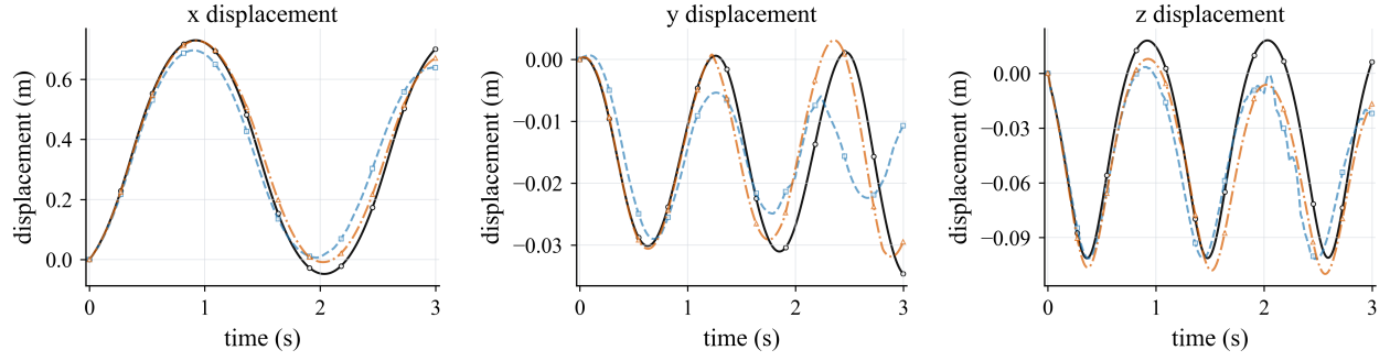
Figure 14: Guide slot validation over 3 s: ball displacement in the x , y , and z directions. The CALG result is shown as the black solid curve; displacements are relative to each solver's initial ball coordinate.
