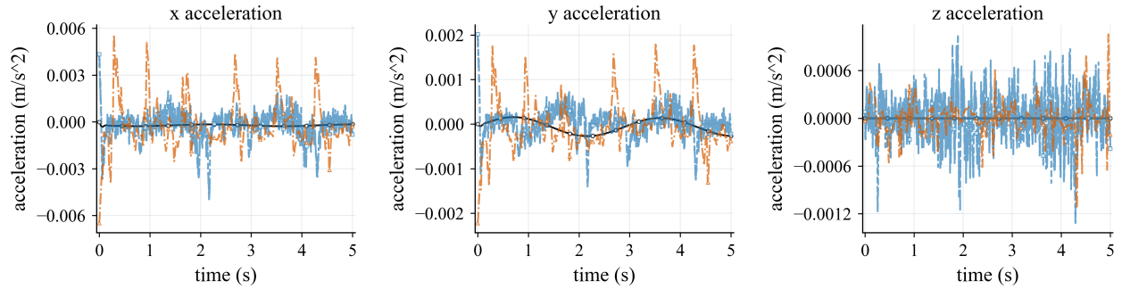
Figure 22: Bearing raceway validation over 5 s: ball acceleration in the x , y , and z directions. For CALG and Recurdyn, acceleration is taken from the exported solver channels; for Chrono it is evaluated from the reported contact force. The plotted curves use a 41-frame centered average for visualization.
