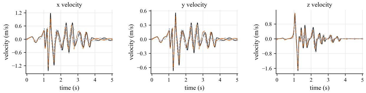
Figure 18: Ball-and-socket pendulum validation over 5 s: ball velocity in the x , y , and z directions. The dominant motion trend is consistent across Chrono, Recurdyn, and CALG, while re-contact transients remain solver dependent.
