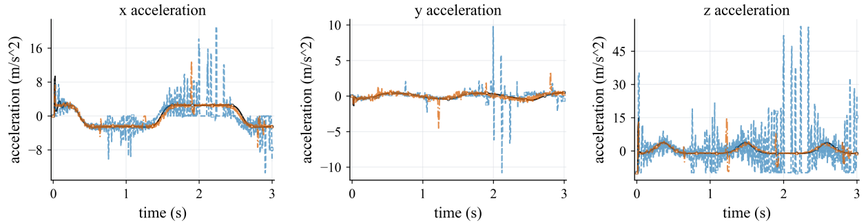
Figure 16: Guide slot validation over 3 s: ball acceleration in the x , y , and z directions. For CALG, acceleration is the effective per-step value exported by the C++ backend after the normal-constraint and gap-clamp update; for Chrono it is evaluated from the reported contact force and gravity; for Recurdyn it is taken from the exported body-acceleration channels. The plotted curves use a 21-frame centered average for visualization.
