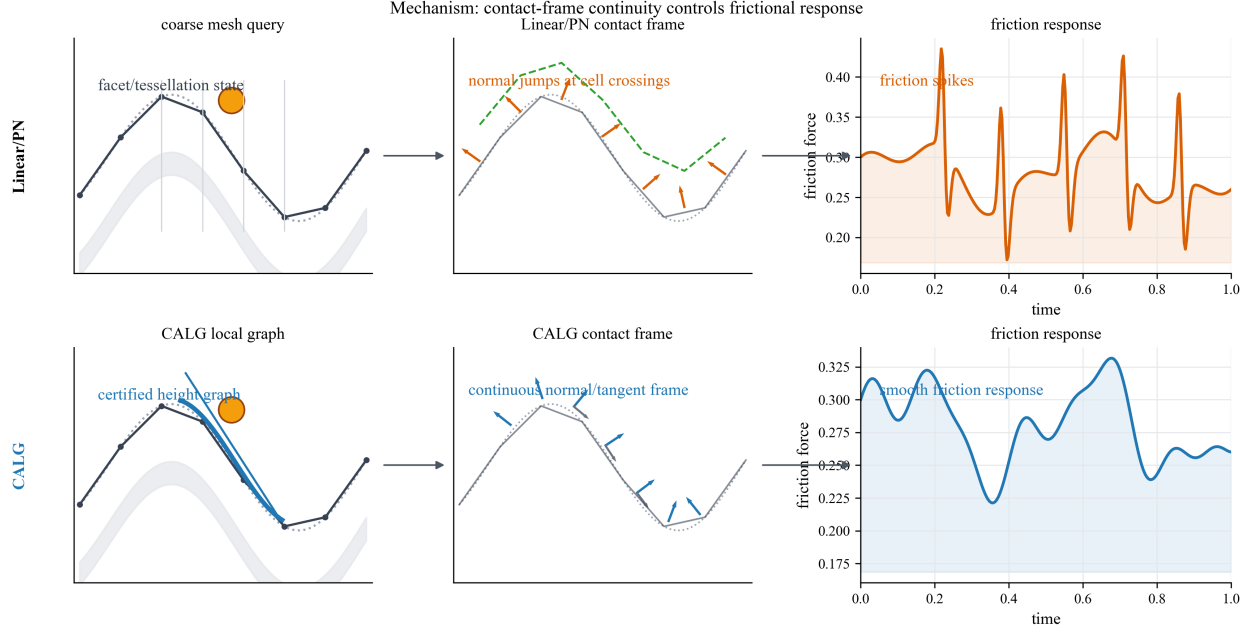
Figure 5: Mechanism-level comparison between facet-based contact-geometry modules and CALG-SDF. Linear-triangle BVH and fixed-tessellation PN-triangle BVH inherit cell-crossing changes in the contact normal or tangent frame, which can enter the regularized Coulomb response as force spikes. CALG instead certifies a contact-aligned local height graph and returns a smooth normal and tangent frame, producing a smoother friction response in the same rigid-body update.
