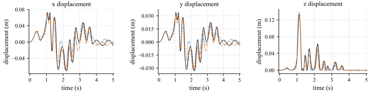
Figure 17: Ball-and-socket pendulum validation over 5 s: ball displacement in the x , y , and z directions. The Recurdyn model uses an equivalent distal payload with the same rod-plus-cylinder mass center and inertia as the Chrono and CALG composite body. The CALG result is shown as the black solid curve; displacements are relative to each solver's initial ball coordinate.
