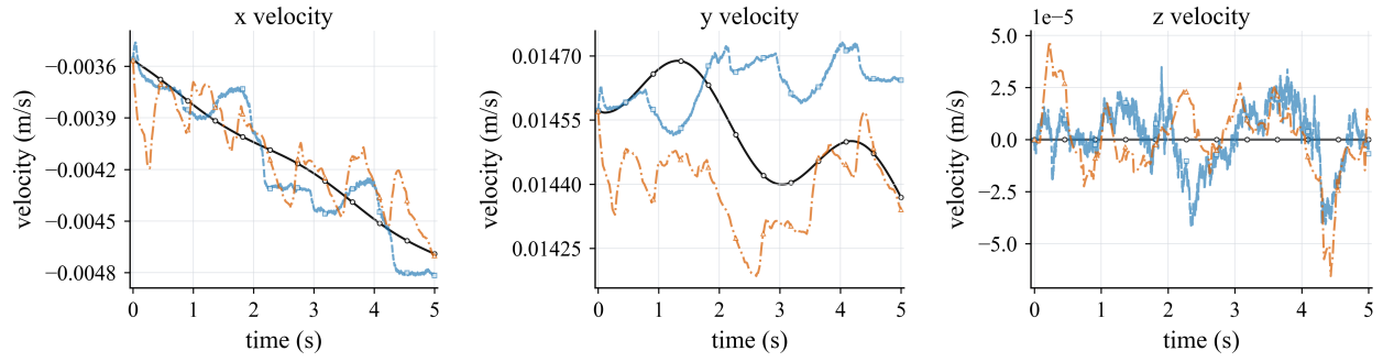
Figure 21: Bearing raceway validation over 5 s: ball velocity in the x , y , and z directions. The CALG result is shown as the black solid curve.
