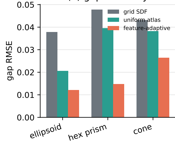
(a) gap accuracy
