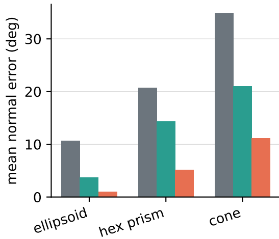
(b) normal accuracy
