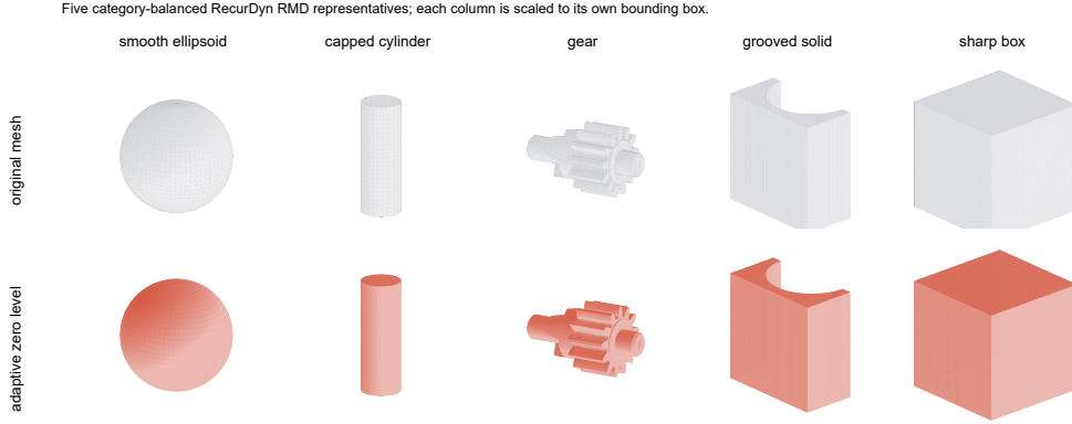
Figure 7: Category-balanced RMD representatives selected from the parsed inventory. The upper row shows the original imported triangle meshes and the lower row shows the feature-adaptive atlas zero-level surface rendered with the same camera for each column. Each column is scaled to its own bounding box so that geometry type and feature coverage are visible; scale is not compared across columns.
