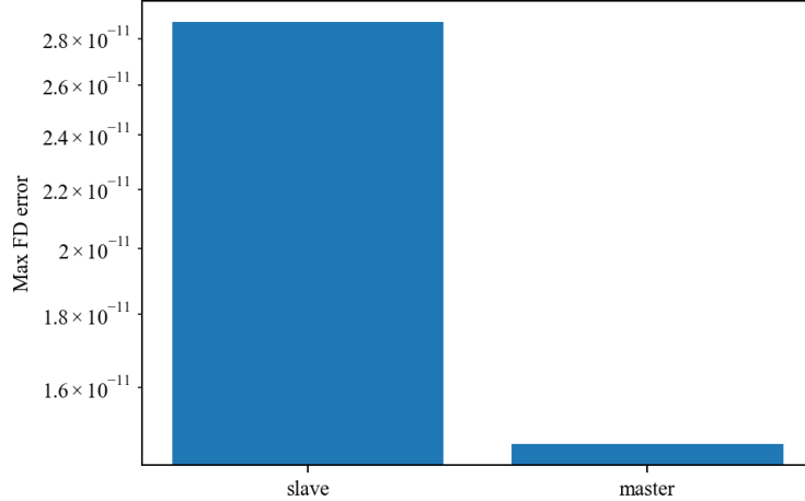
Figure 3: Slave and master field-contact Jacobian finite-difference errors.
