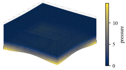
Contact pressure and scalar-gradient normals (81 active samples)
