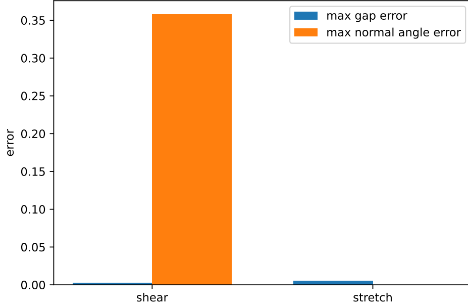
Figure 12: Material-space SDF baseline error under stretch and shear. The proposed method queries the current FEM surface; the baseline carries a frozen material-space distance.
