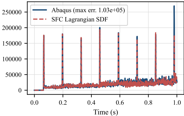
P95 stress history
