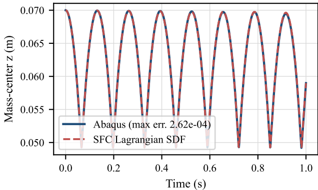
Full sphere-drop trajectory
