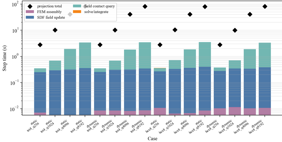
Figure 9: Solver-level timing breakdown for TET4/HEX8 static and dynamic contact-dominated workloads. Diamonds mark the projection-reference total step time.
