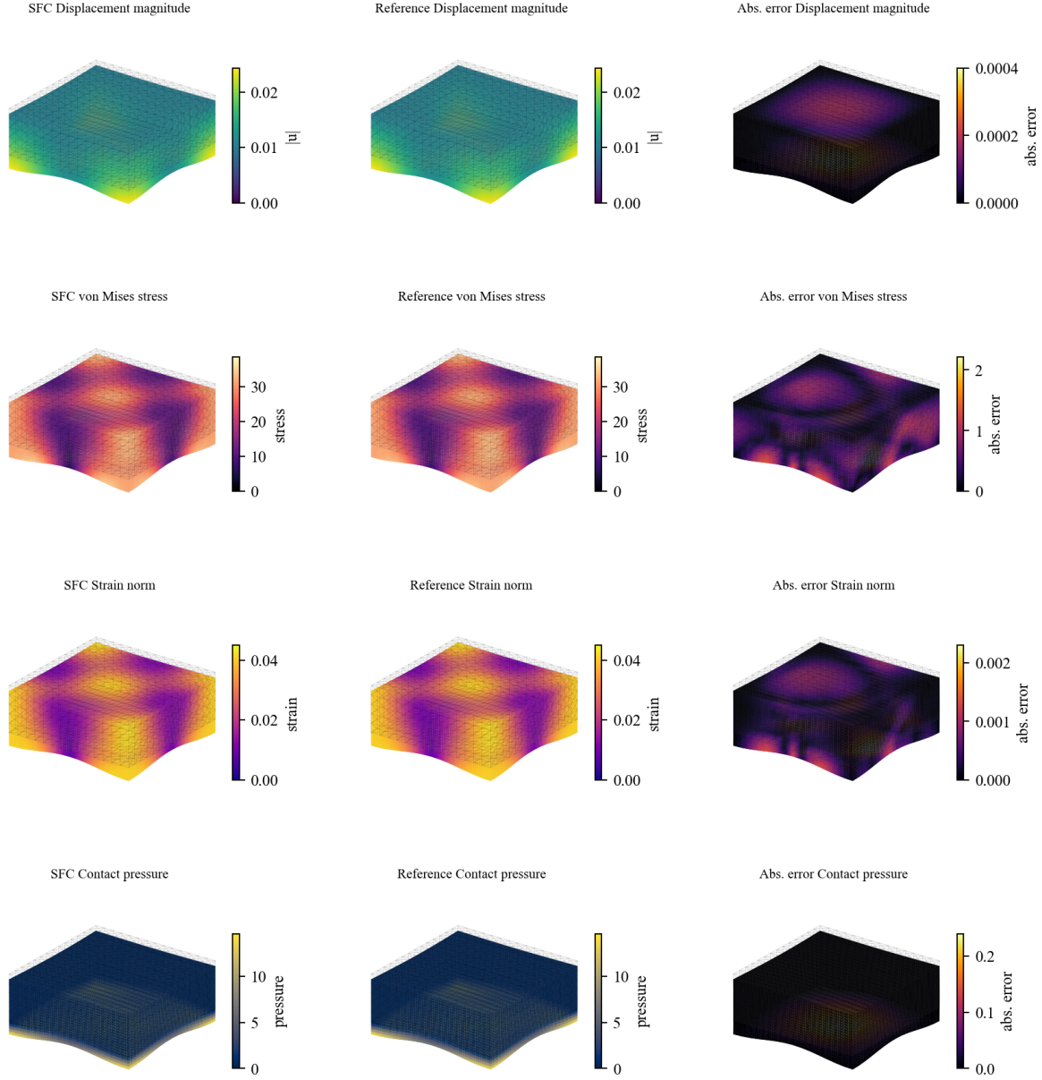
Figure 12: External visual FEM validation rendered on the deformed three-dimensional boundary surface. Each row compares SFC, generated reference, and absolute error with matched SFC/reference color scales and a deformation scale of 4x.
