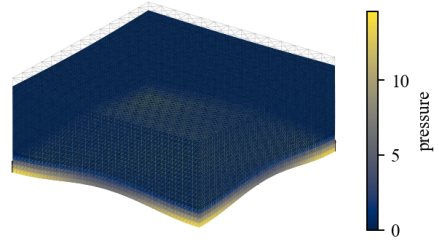
Contact pressure and scalar-gradient normals (225 active samples)
