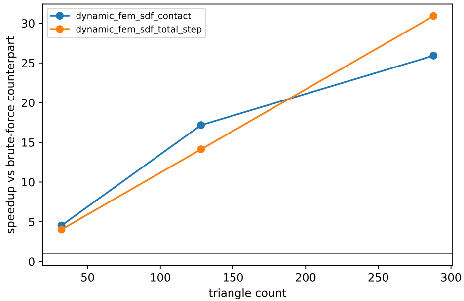
Figure 13: Phase-7 acceleration feasibility. The plot separates contact-only speedup from total-step speedup that includes FEM assembly and a sparse linear solve.
