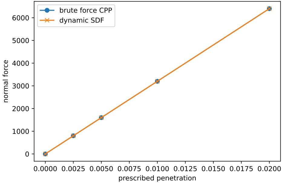
Figure 8: Contact force-displacement comparison against brute-force closest-point projection contact. The curves overlap for the tested rigid-plane normal penalty case.
