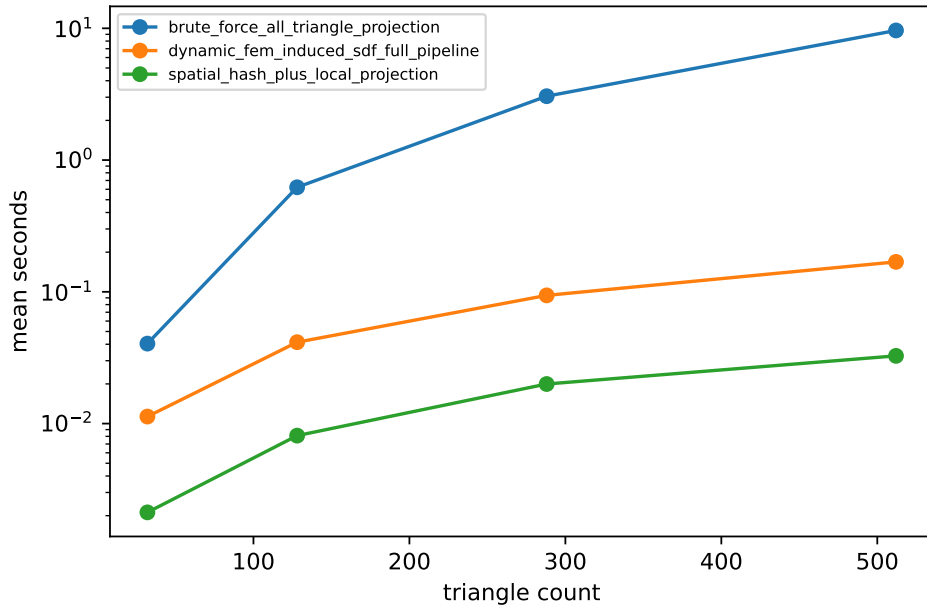
Figure 11: Performance scaling for brute-force all-triangle projection, spatial-hash plus local projection, and the dynamic FEM-induced SDF full pipeline.
