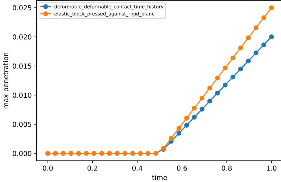
Figure 10: Contact time-history diagnostics from the Phase-6 package. The plotted quantities summarize penetration behavior for the rigid-plane and deformable-deformable contact checks.
