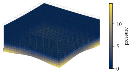
Contact pressure and scalar-gradient normals (81 active samples)
