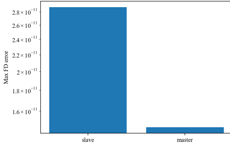
Figure 3: Slave and master field-contact Jacobian finite-difference errors.
