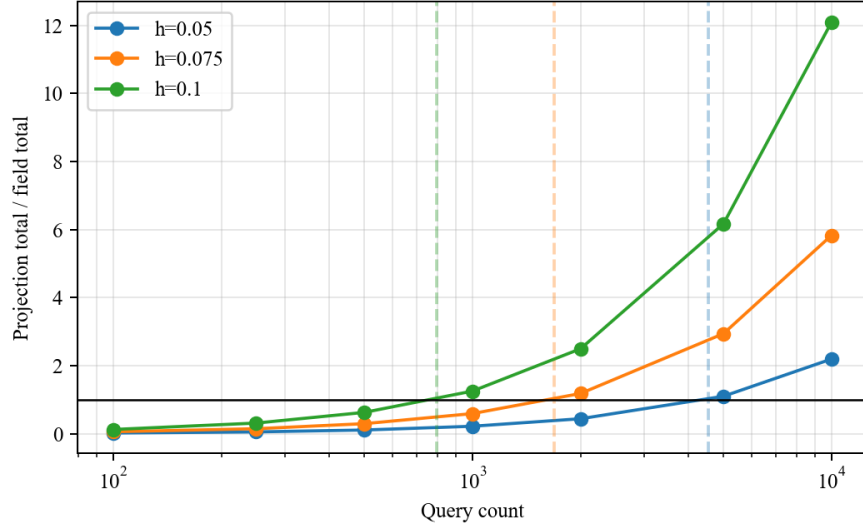
Figure 6: Amortized speedup as projection-query total time divided by SDF-field total time. Dashed vertical markers indicate measured crossover counts.
