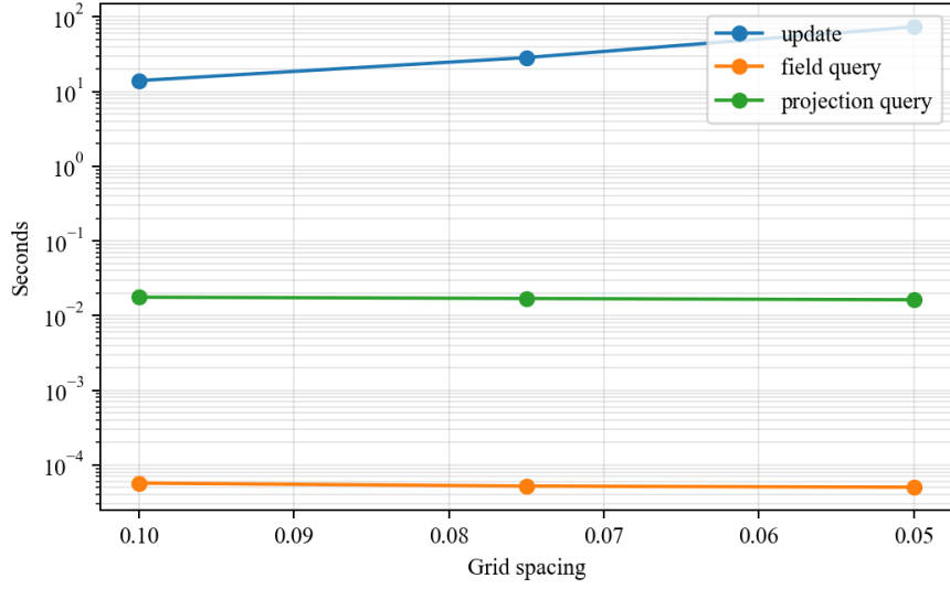
Figure 5: Field update, field query, and projection query timing components.
