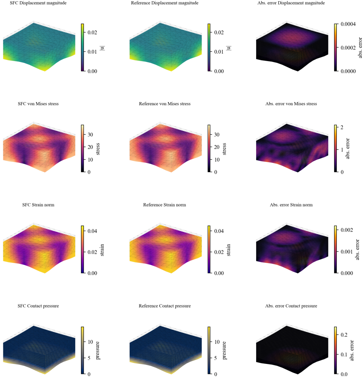
Figure 8: External visual FEM validation rendered on the deformed three-dimensional boundary surface. Each row compares SFC, generated reference, and absolute error with matched SFC/reference color scales and a deformation scale of 4 \times .
