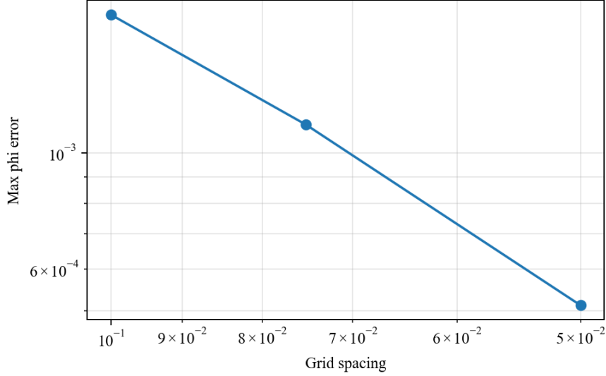
Figure 1: Field \phi error decreases with grid spacing for the tested nonplanar surface.
