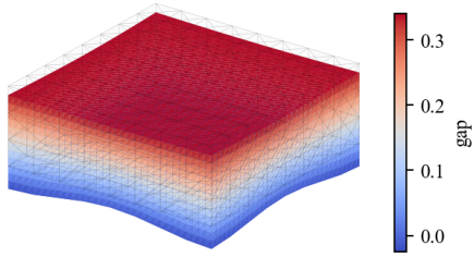
Current FEM surface colored by interpolated gap
