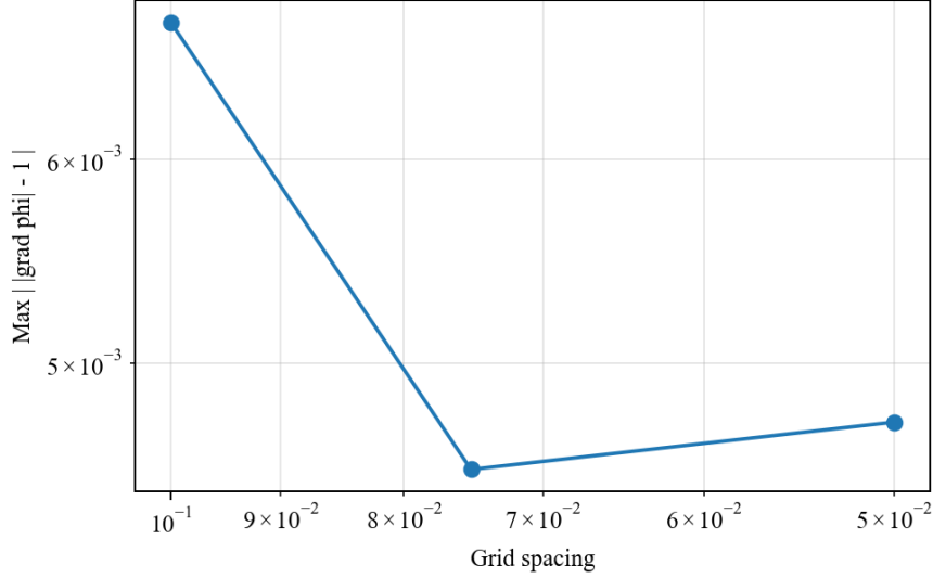
Figure 2: Maximum Eikonal residual over the dynamic narrow band.
