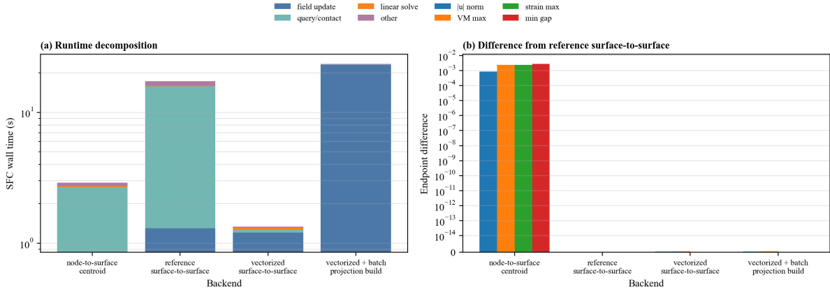
Figure 16: Representative backend ablation for node-to-surface sampling, reference surface-to-surface quadrature, vectorized surface-to-surface quadrature, and vectorized field contact with forced batch projection during field construction. The legend is placed outside the axes so the timing bars and endpoint-difference bars remain unobstructed.
