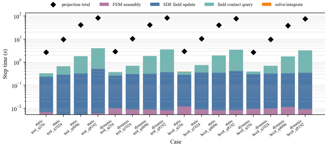
Figure 14: Solver-level timing breakdown for TET4/HEX8 static and dynamic contact-dominated workloads. Diamonds mark the projection-reference total step time.
