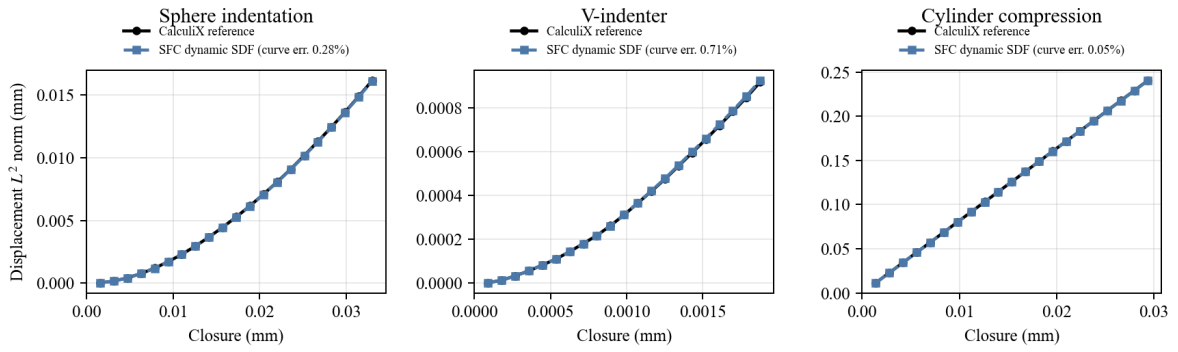
Figure 9: Quasi-static closure/load displacement-norm trajectories for independent CalculiX native contact and SFC dynamic-SDF contact. Each case uses 21 closure steps, and each SFC legend reports the full-curve displacement L^2 relative error.
