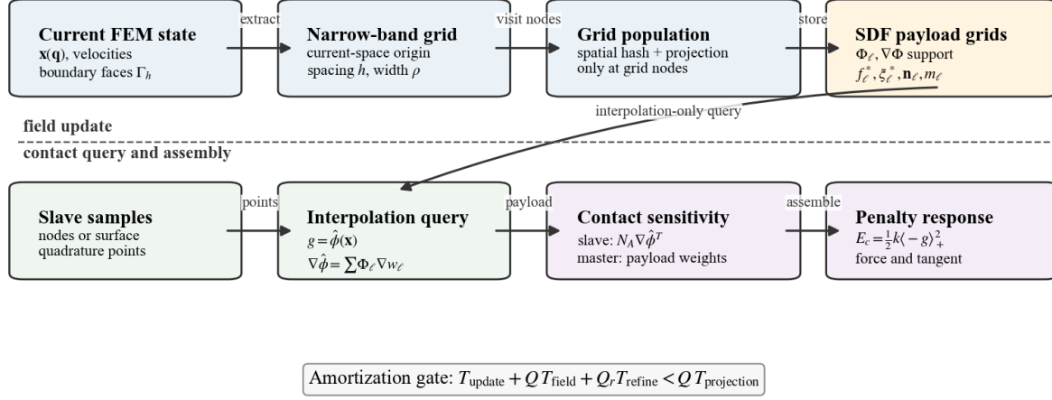
Figure 1: Compact architecture of the dynamic narrow-band SDF update and field-contact query. The upper row is the current-configuration field update, where projection is used only to populate grid-node values and closest-feature payloads. The lower row is the repeated contact path, which evaluates gaps, scalar-field derivatives, Jacobians, and penalty forces by interpolation.
