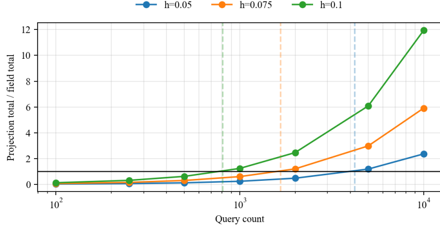
Figure 7: Amortized speedup as projection-query total time divided by SDF-field total time. Dashed vertical markers indicate measured crossover counts.
