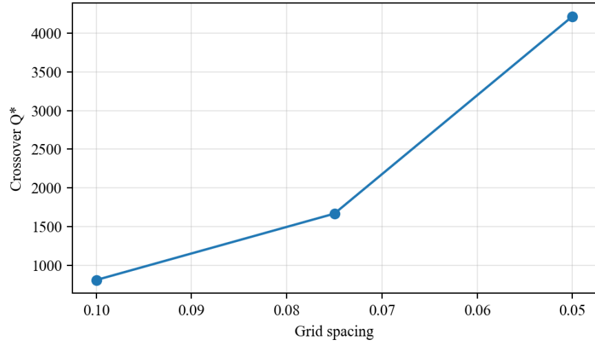
Figure 8: Measured crossover query count Q^* for each grid spacing.
