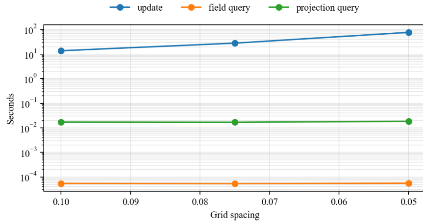
Figure 6: Field update, field query, and projection query timing components.
