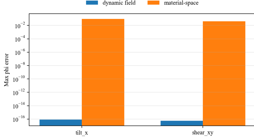
Figure 5: Material-space SDF error under current-surface deformation compared with the rebuilt dynamic field.
