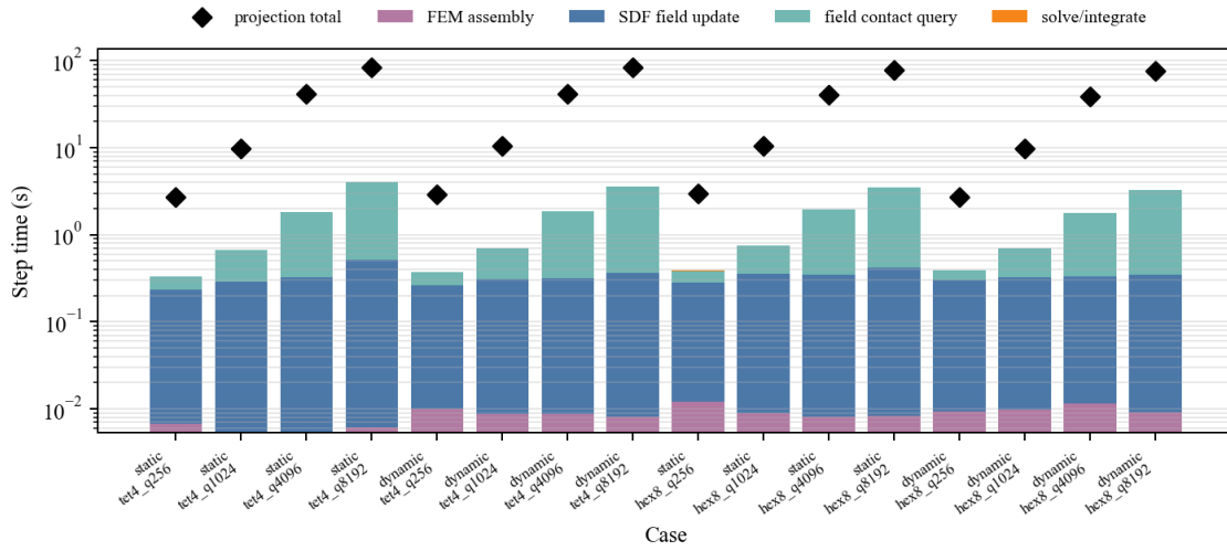
Figure 13: Solver-level timing breakdown for TET4/HEX8 static and dynamic contact-dominated workloads. Diamonds mark the projection-reference total step time.
