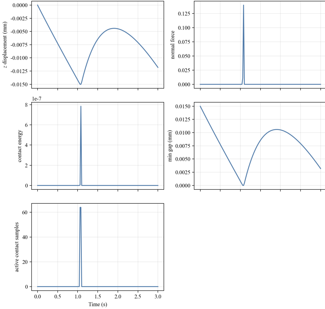
Figure 9: Three-second C3D8 dynamic SDF-contact time histories. The horizontal axis is physical time; the outputs are z -displacement, normal force, contact energy, minimum gap, and active contact sample count.
