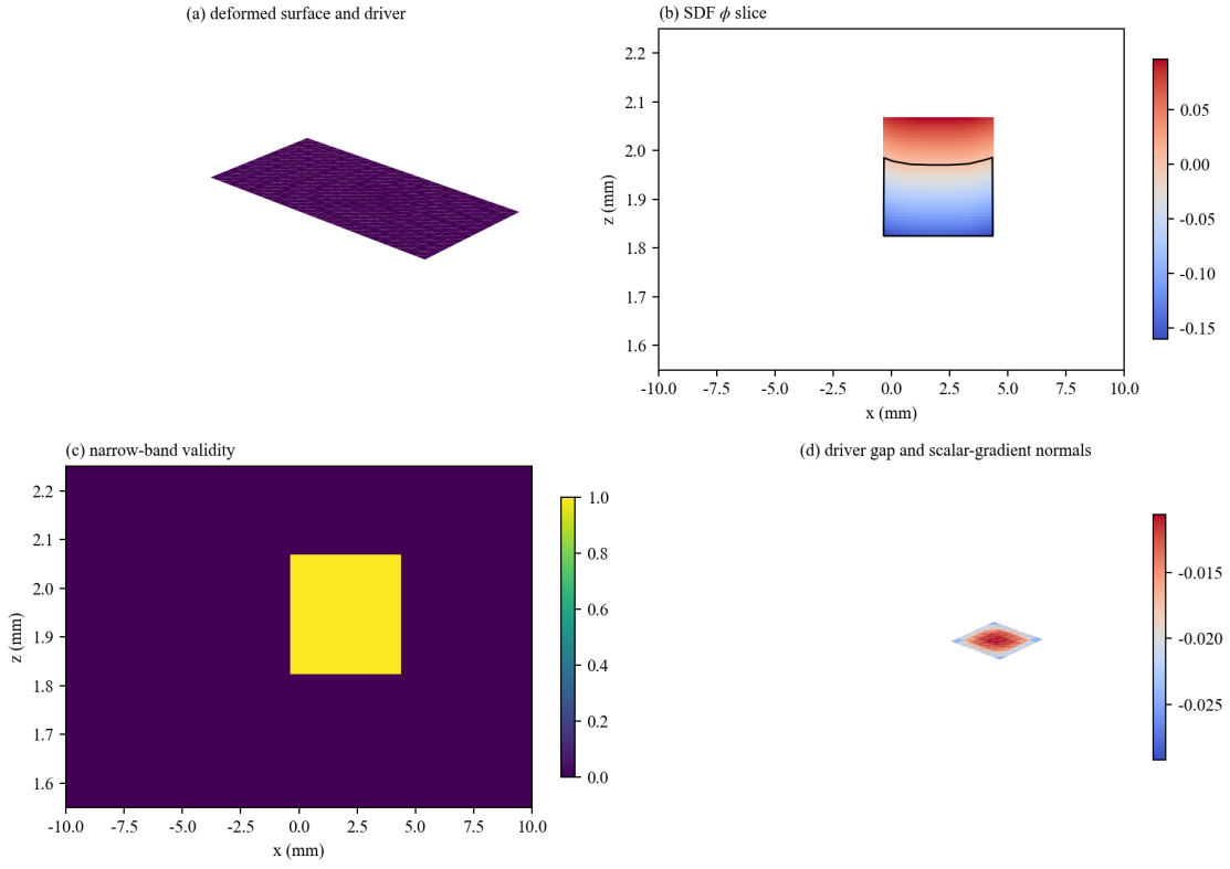
Figure 12: SDF-field visualization for the Fig. 6-inspired case: deformed contact surface and driver, \phi slice with zero contour, narrow-band validity, and driver gap with scalar-gradient normals.
