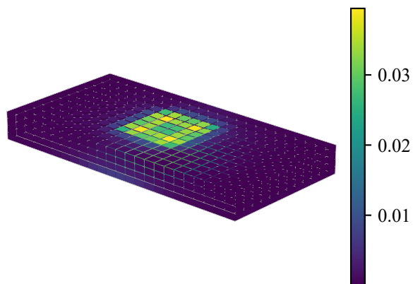
strain norm
