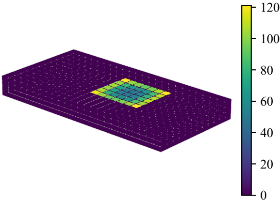
contact pressure
