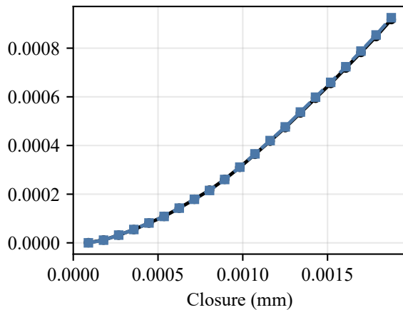
V-indenter ● CalculiX reference ■ SFC dynamic SDF (curve err. 0.71%)
