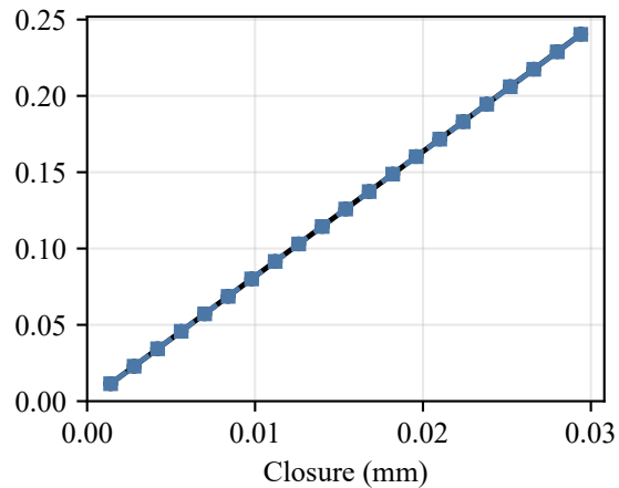
Cylinder compression ● CalculiX reference ■ SFC dynamic SDF (curve err. 0.05%)
