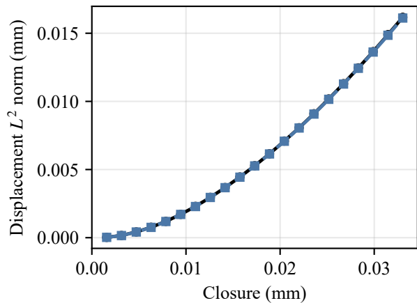
Sphere indentation ● CalculiX reference ■ SFC dynamic SDF (curve err. 0.28%)
