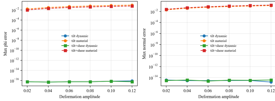
Figure 4: Material-space SDF error under increasing current-surface deformation compared with the rebuilt dynamic field. Solid lines denote the rebuilt dynamic field and dashed lines denote the frozen material-space field.
