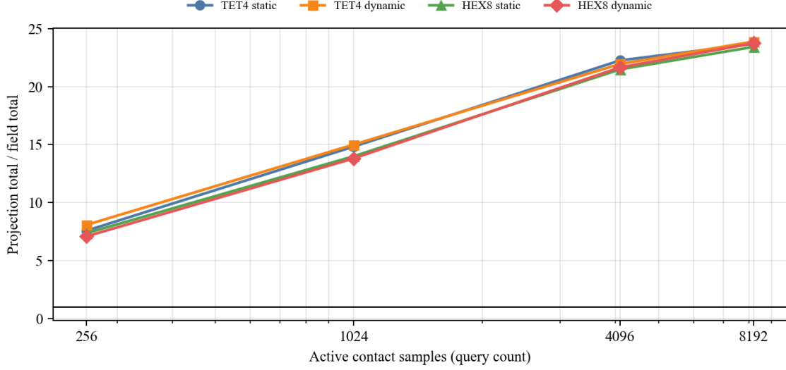
Figure 14: Projection-reference total step time divided by true-field total step time as a function of active contact samples. This curve form exposes the amortized SDF-query advantage more directly than a case-indexed speedup bar chart.
