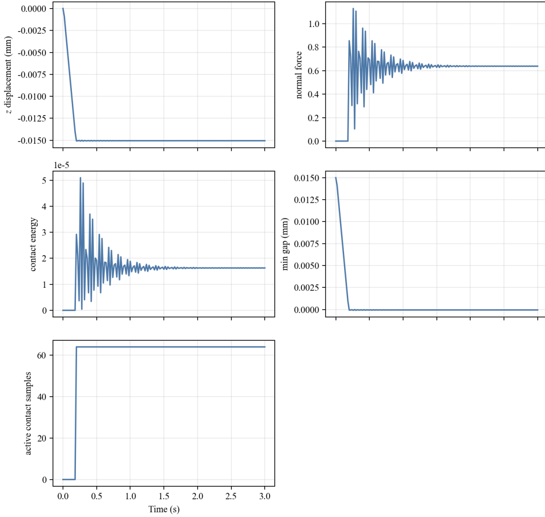
Figure 10: Three-second C3D8 free-fall settling SDF-contact time histories. The horizontal axis is physical time; the outputs are z -displacement, normal force, contact energy, minimum gap, and active contact sample count.
