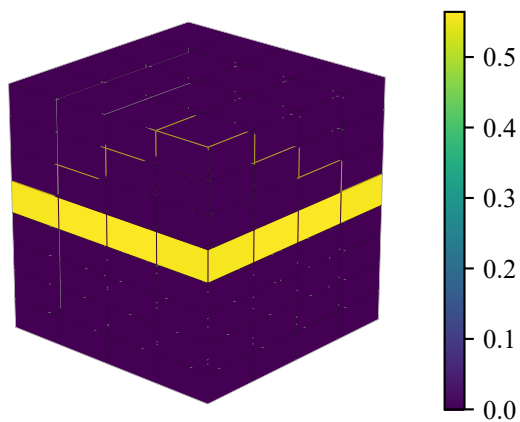
contact pressure
