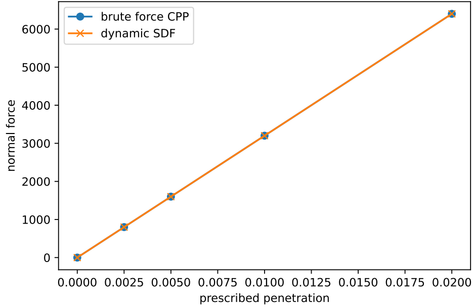
Figure 16: Contact force-displacement comparison against brute-force closest-point projection contact. The curves overlap for the tested rigid-plane normal penalty case.
