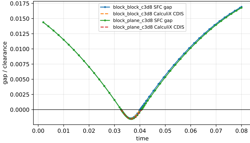
Figure 10: C3D8 dynamic contact trajectory replay: SFC current-surface dynamic-SDF gap compared with CalculiX CDIS output where contact rows are available.
