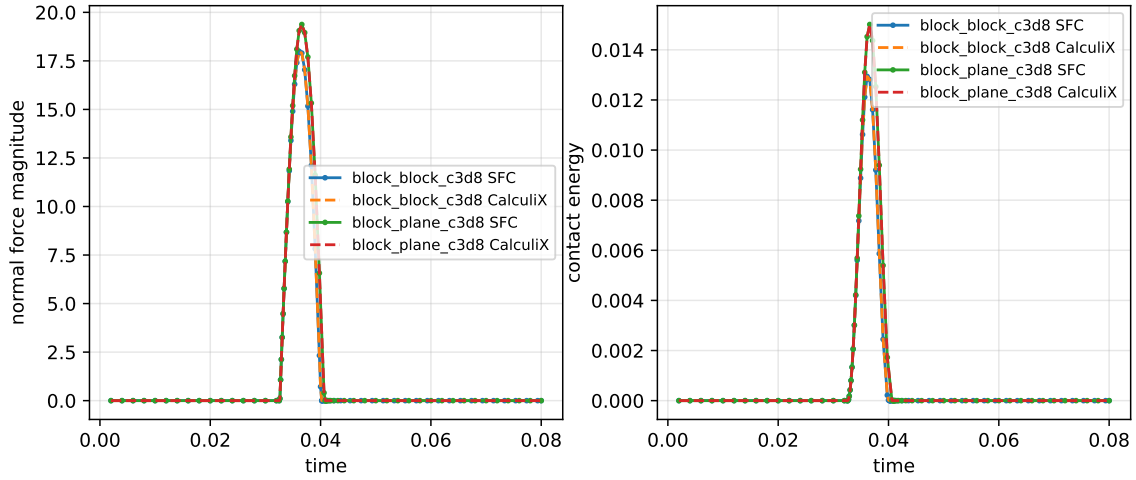
Figure 11: C3D8 dynamic contact trajectory replay: fixed-support reaction force and contact spring energy from CalculiX compared with the SFC dynamic-SDF replay force and penalty energy.
