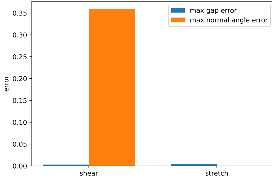
Figure 17: Material-space SDF baseline error under stretch and shear. The proposed method queries the current FEM surface; the baseline carries a frozen material-space distance.
