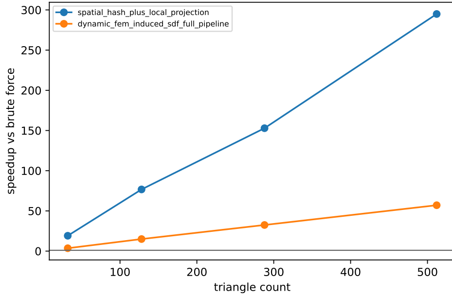
Figure 20: Measured speedup against brute-force all-triangle projection for the tested surface resolutions.
