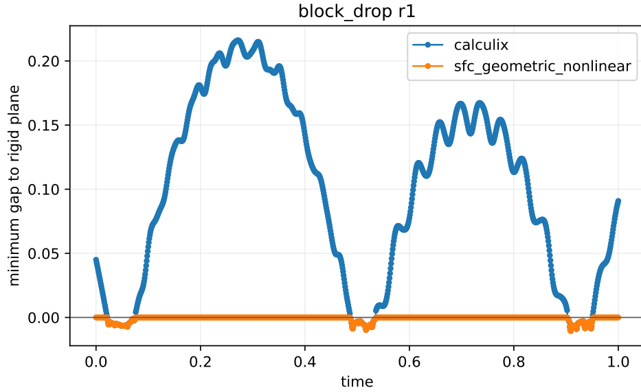
Figure 14: Minimum contact gap history in the dynamic CalculiX comparison. The plot reports the penetration behavior produced by the dynamic-SDF contact backend and the CalculiX reference output.
