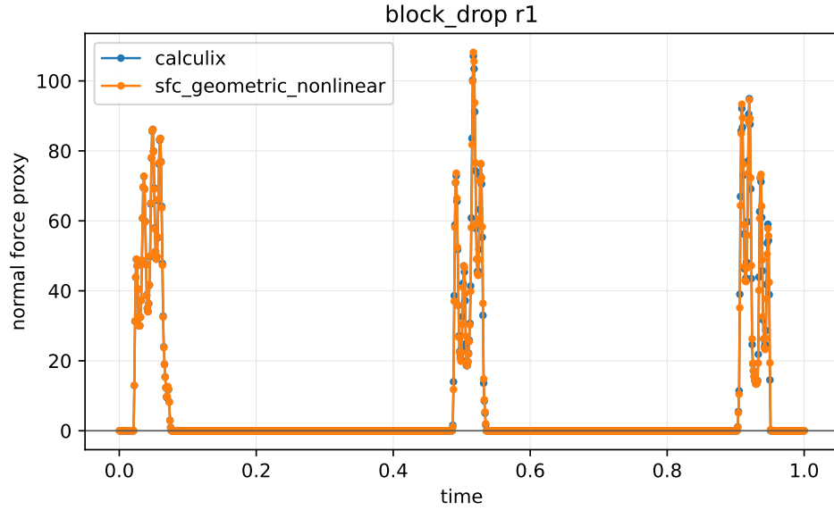
Figure 15: Normal reaction force history for the locked dynamic block-plane comparison. Force agreement is evaluated using CalculiX reaction/contact output where available.
