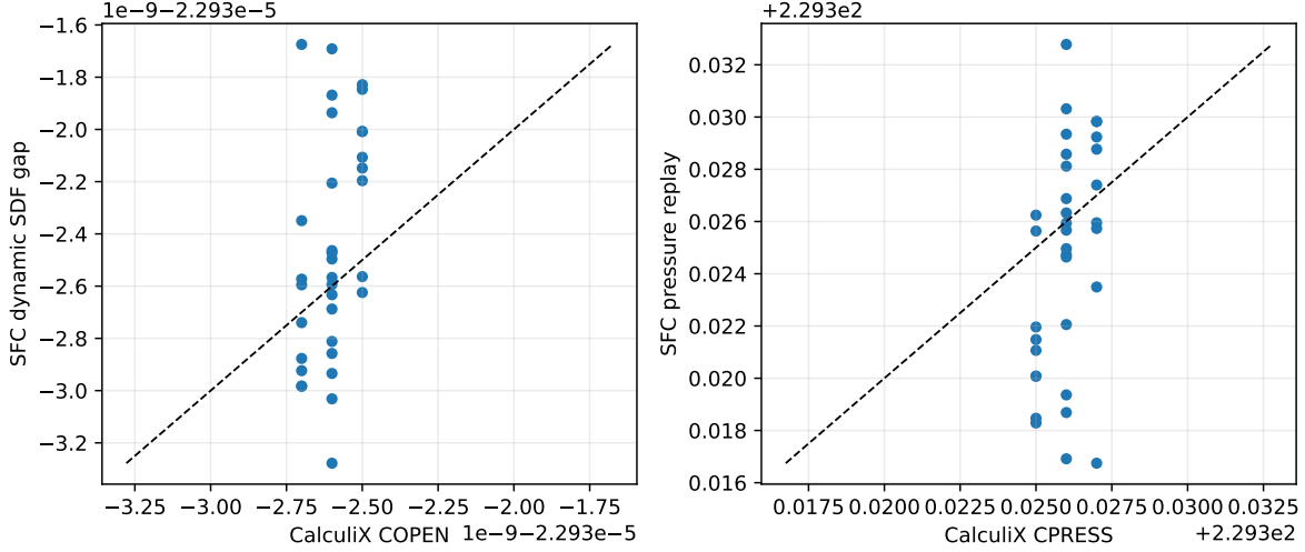
Figure 6: Official scheibe2f2f FRD replay. SFC recomputes the current-surface dynamic-SDF gap and linear pressure-overclosure response from the CalculiX final deformed C3D8 master surface.
