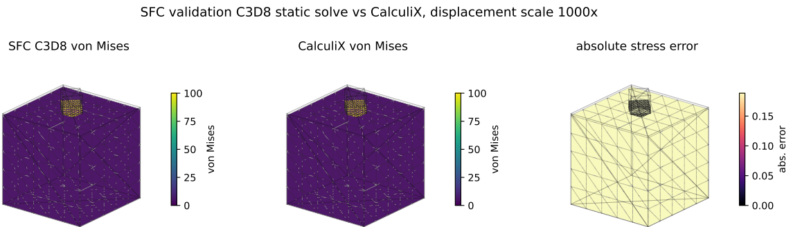
Figure 9: Direct validation-only C3D8 comparison on CalculiX contactenergy.inp . The first panel shows the SFC C3D8 static solve, the second shows CalculiX, and the third shows the absolute von Mises stress error. This comparison is included to make the external contact evidence visually auditable; it is not a claim of nonlinear C3D8 dynamic trajectory equivalence.
