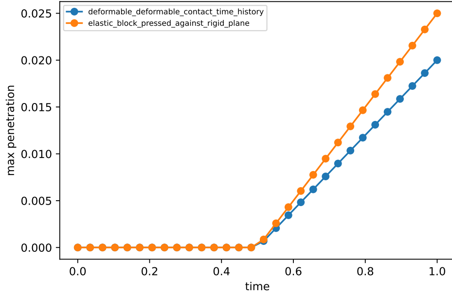
Figure 18: Contact time-history diagnostics from the Phase-6 package. The plotted quantities summarize penetration behavior for the rigid-plane and deformable-deformable contact checks.
