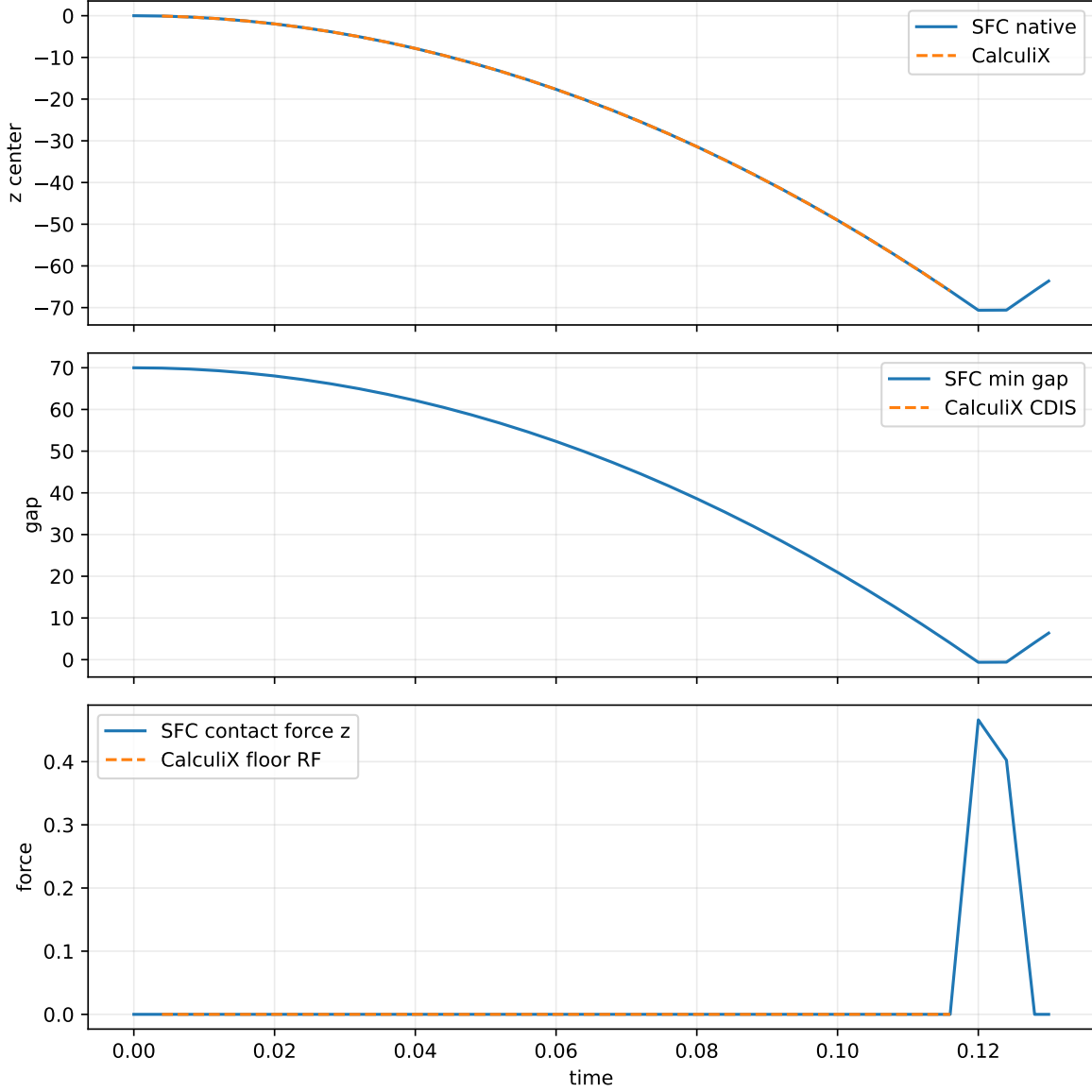
Figure 7: Official ball dynamic-drop probe. The SFC native C3D8 trajectory agrees with CalculiX in the exported pre-contact center trajectory. SFC then reaches first contact and rebounds, while the locked CalculiX run fails near first contact and therefore does not support a full contact-trajectory equivalence claim.
