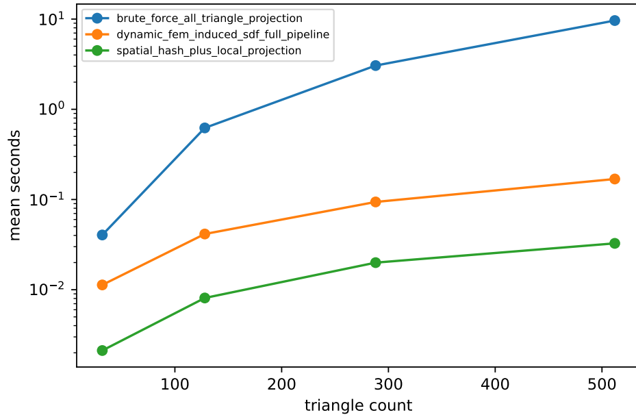
Figure 19: Performance scaling for brute-force all-triangle projection, spatial-hash plus local projection, and the dynamic FEM-induced SDF full pipeline.
