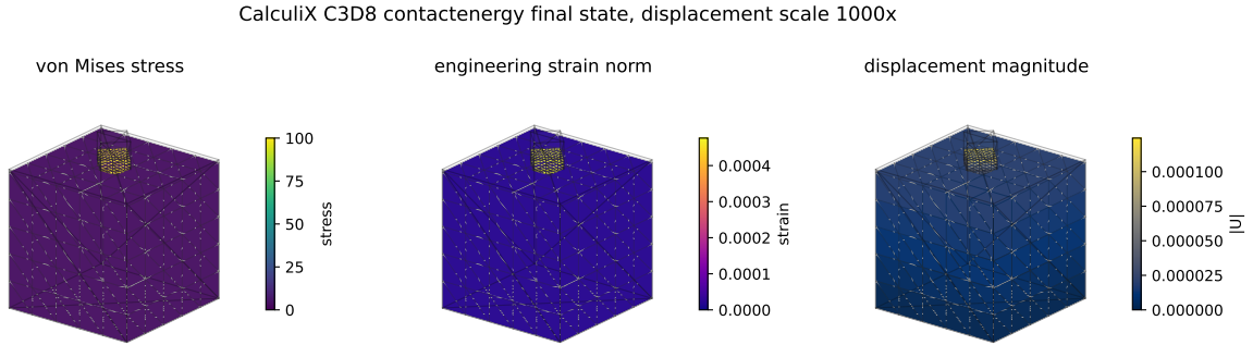
Figure 8: CalculiX contactenergy.inp C3D8 final-state visualization. The stress and strain fields are post-processed from the final CalculiX displacement field, averaged to boundary nodes, and interpolated over triangulated C3D8 boundary faces. The deformed shape is plotted with a labeled displacement scale factor to make the small static deformation visible.
