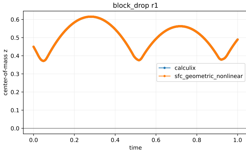
Figure 13: Dynamic block-plane center-of-mass trajectory compared against CalculiX for the locked 1 s contact case.
