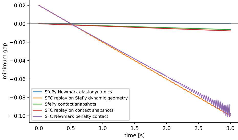
Figure 9: External transient/contact reference. The SfePy transient elastodynamic run provides the 3-second Newmark/mass reference, while SfePy contact snapshots and SFC replay compare contact activation and gap scale along the same path.
