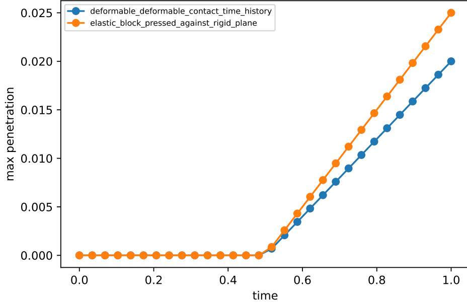
Figure 12: Contact time-history diagnostics from the Phase-6 package. The plotted quantities summarize penetration behavior for the rigid-plane and deformable-deformable contact checks.
