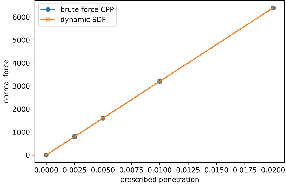
Figure 10: Contact force-displacement comparison against brute-force closest-point projection contact. The curves overlap for the tested rigid-plane normal penalty case.
