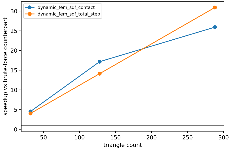
Figure 15: Phase-7 acceleration feasibility. The plot separates contact-only speedup from total-step speedup that includes FEM assembly and a sparse linear solve.
