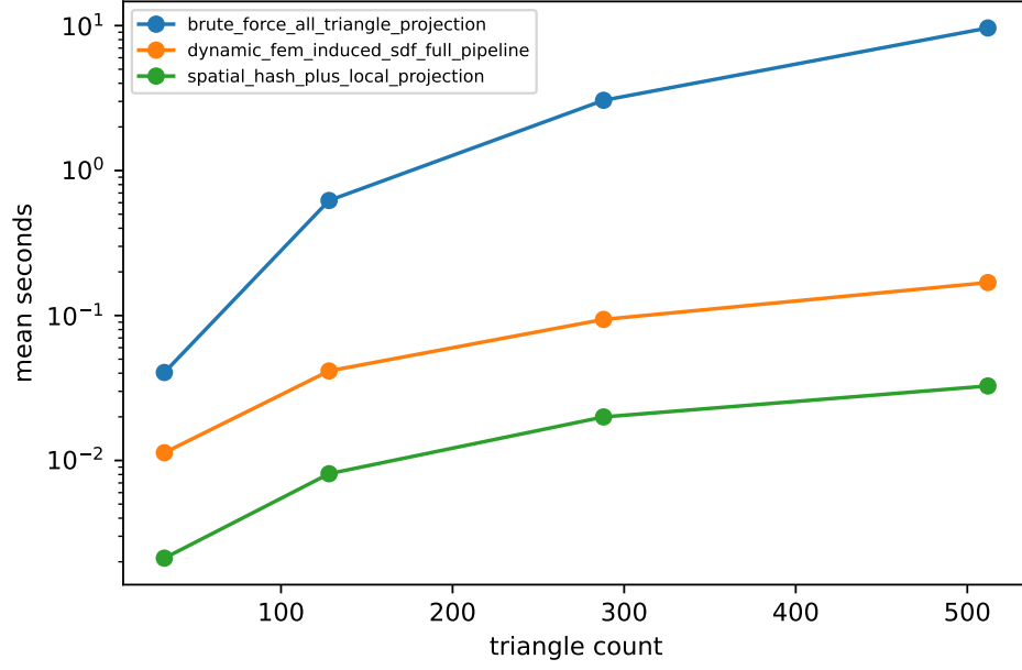
Figure 13: Performance scaling for brute-force all-triangle projection, spatial-hash plus local projection, and the dynamic FEM-induced SDF full pipeline.
