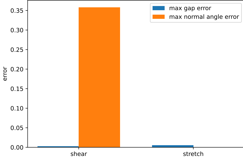
Figure 15: Material-space SDF baseline error under stretch and shear. The proposed method queries the current FEM surface; the baseline carries a frozen material-space distance.
