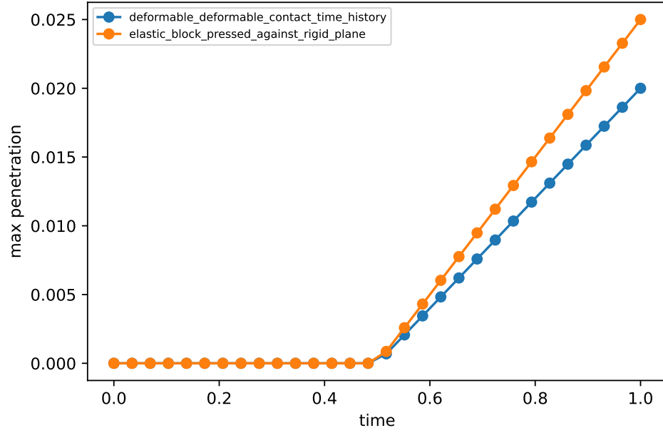
Figure 16: Contact time-history diagnostics from the Phase-6 package. The plotted quantities summarize penetration behavior for the rigid-plane and deformable-deformable contact checks.
