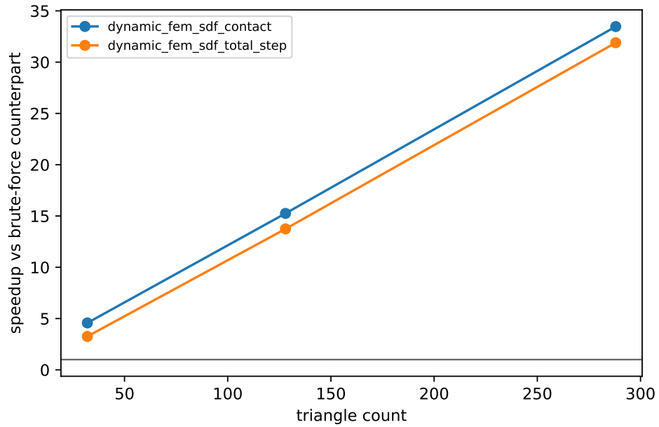
Figure 19: Phase-7 acceleration feasibility. The plot separates contact-only speedup from total-step speedup that includes FEM assembly and a sparse linear solve.
