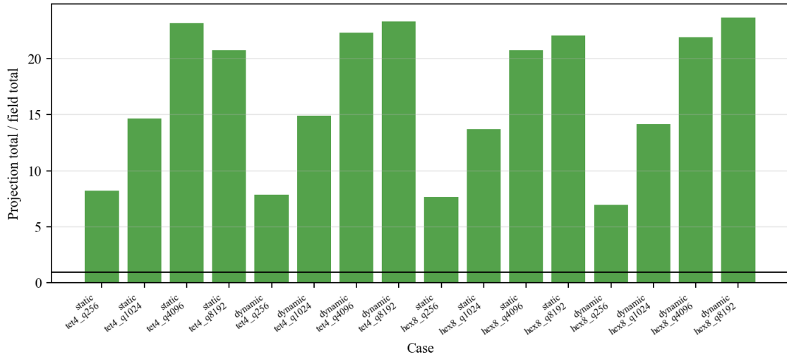
Figure 11: Projection-reference total step time divided by true-field total step time for the solver-level timing cases.
