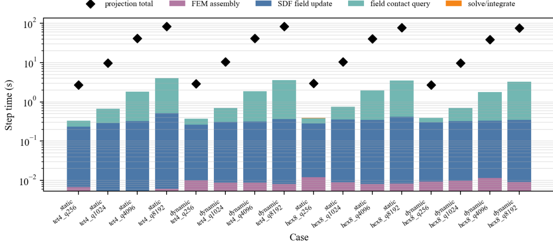
Figure 10: Solver-level timing breakdown for TET4/HEX8 static and dynamic contact-dominated workloads. Diamonds mark the projection-reference total step time.
