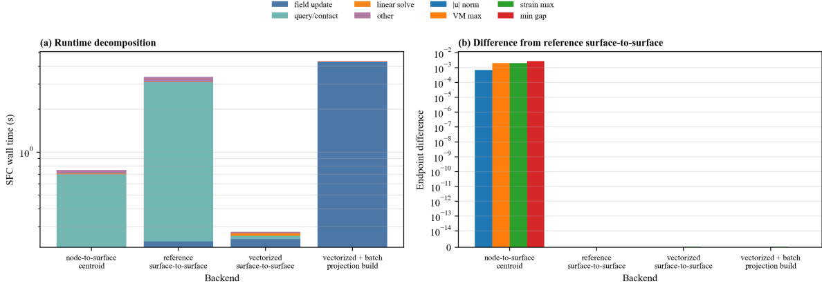
Figure 12: Representative backend ablation for node-to-surface sampling, reference surface-to-surface quadrature, vectorized surface-to-surface quadrature, and vectorized field contact with forced batch projection during field construction. The legend is placed outside the axes so the timing bars and endpoint-difference bars remain unobstructed.
