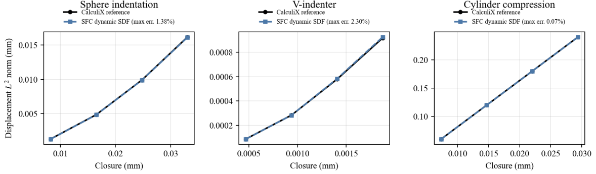
Figure 8: Quasi-static closure/load displacement-norm trajectories for independent CalculiX native contact and SFC dynamic-SDF contact. Each SFC legend reports the maximum displacement-field L^2 relative error for that problem, replacing the earlier error-bar summary with curve-level agreement.
