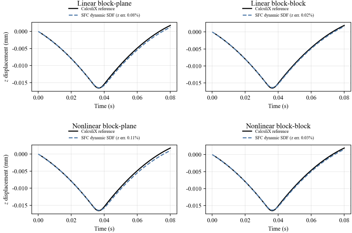
Figure 9: Dynamic C3D8 contact displacement histories. For dynamic simulations the independent variable is physical time; each panel compares the SFC dynamic-SDF contact trajectory with the CalculiX reference, and the SFC legend reports the z -displacement history error.
