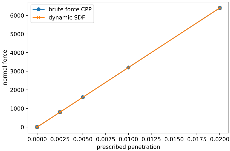
Figure 14: Contact force-displacement comparison against brute-force closest-point projection contact. The curves overlap for the tested rigid-plane normal penalty case.
