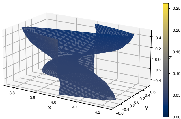
patch residual ILC error
