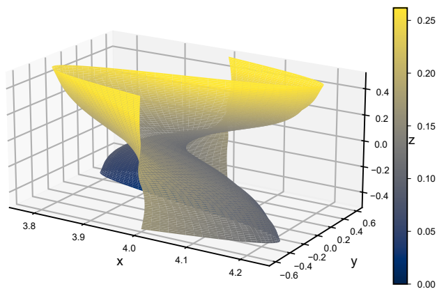
low-mode error
