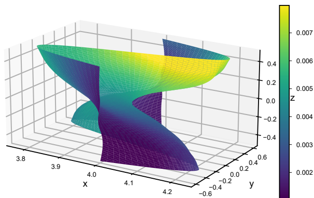
equivalent strain
