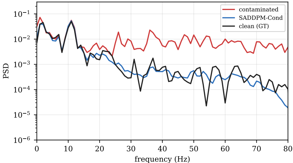
EMG: spectral recovery
