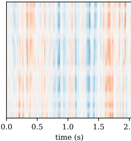
SADDPM-Cond
