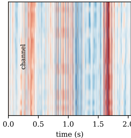
contaminated
