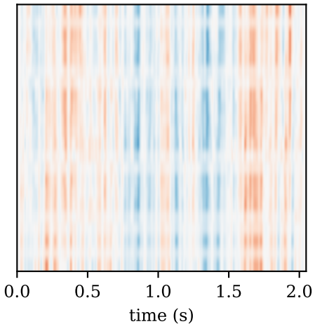
clean (GT)
