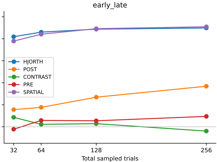
Same 43 identities at every trial budget; split-half reliability is not clinical validity
