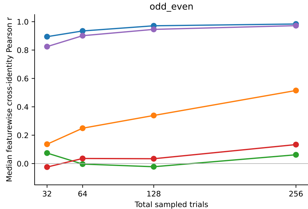
Same 43 identities at every trial budget; split-half reliability is not clinical validity
