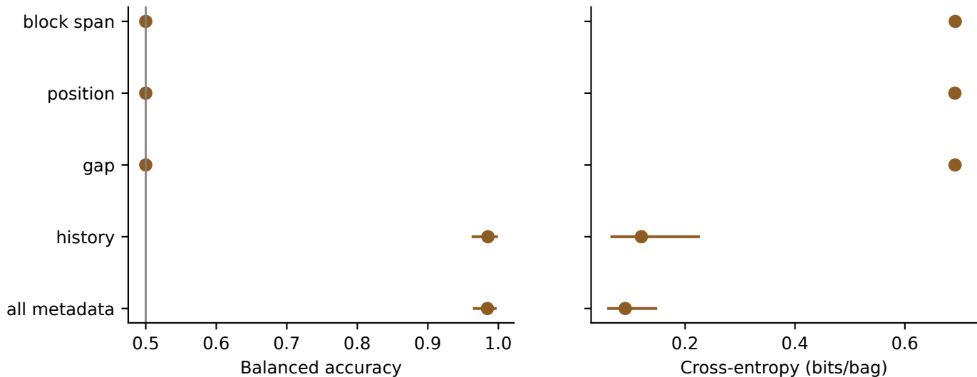
N2: metadata-only diagnostic on original bags (57 identities)
