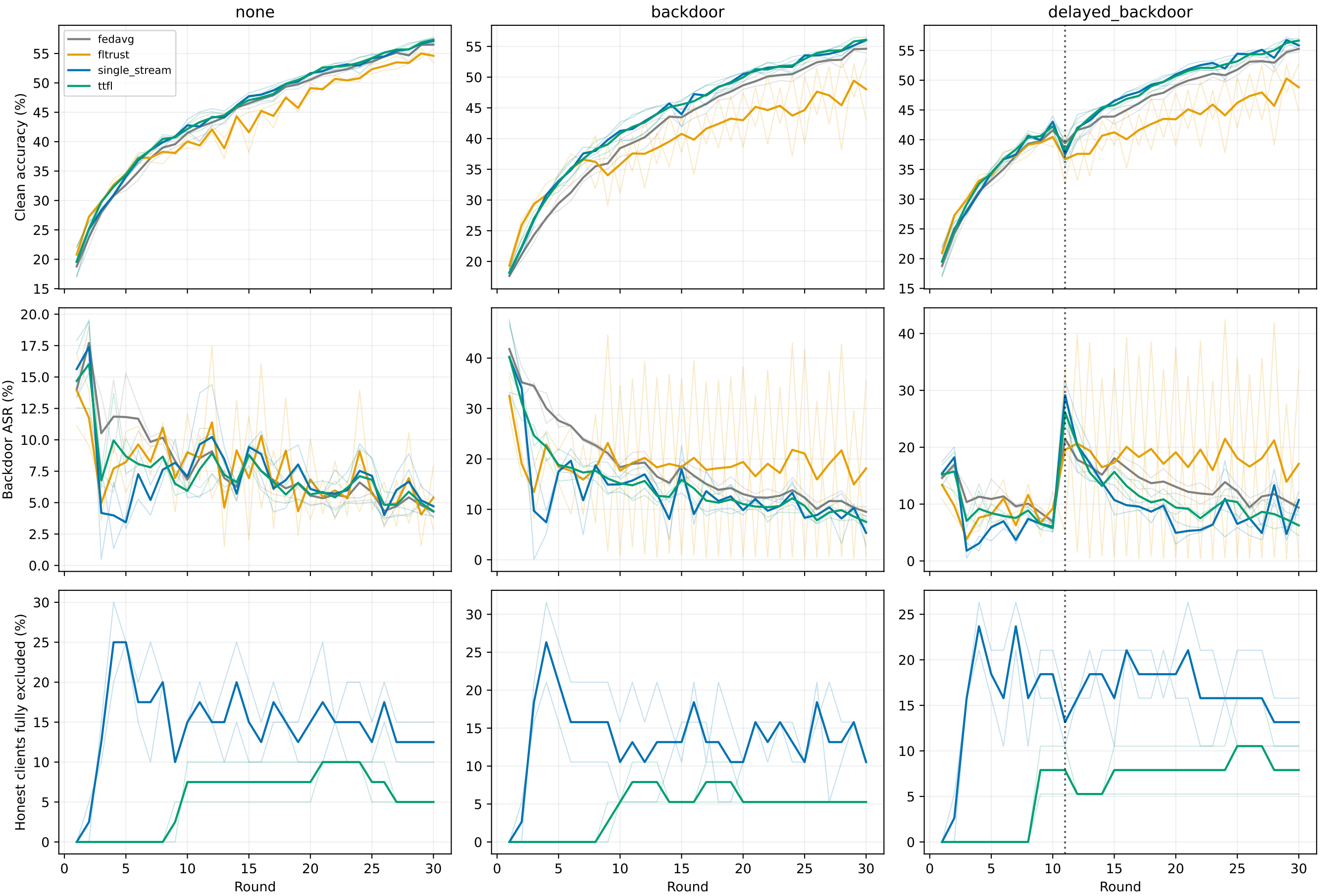
30-round development matrix | 2 seeds | solid: mean; faint: each seed
